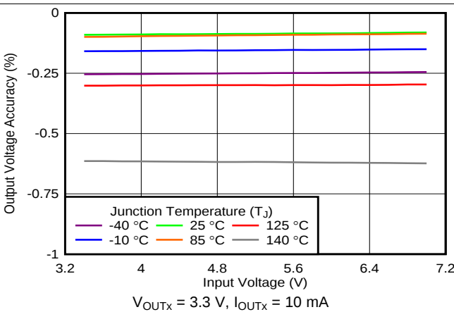
FIG 28. Line Regulation
