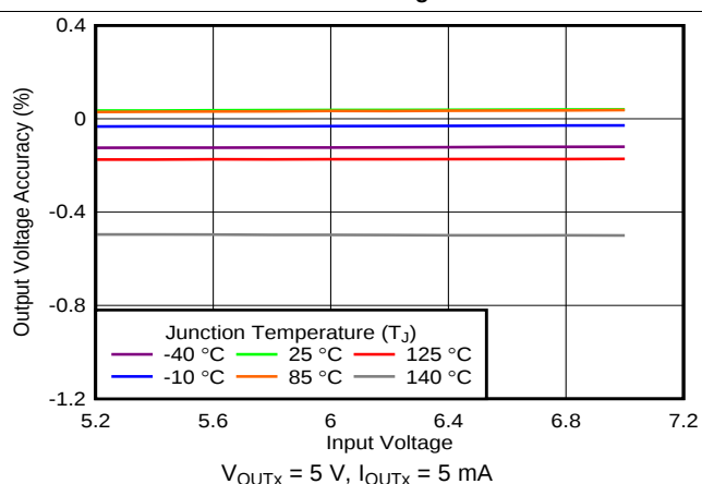
FIG 30. Line Regulation
