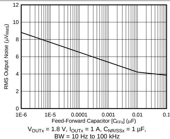
FIG 14. RMS Output Noise vs C_{\text{FFX}}
