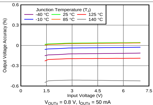
FIG 26. Line Regulation
