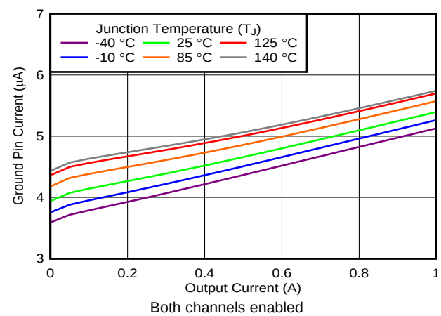
FIG 32. Ground Current vs Output Current
