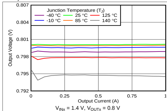
FIG 25. Load Regulation
