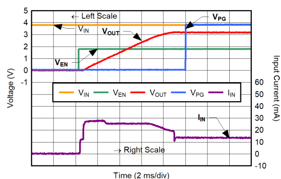
Figure 6-30. Inrush Current for C_{NR/SS} = 4.7\text{ }\mu\text{F}
