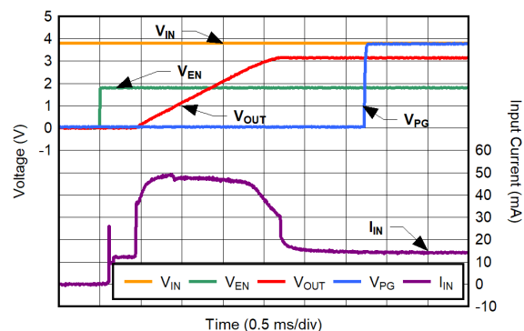
Figure 6-28. Inrush Current for C_{NR/SS} = 1.0\text{ }\mu\text{F}
