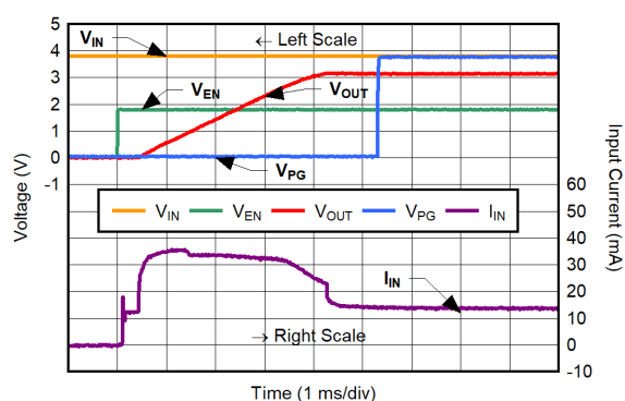
Figure 6-29. Inrush Current for C_{NR/SS} = 2.2\text{ }\mu\text{F}
