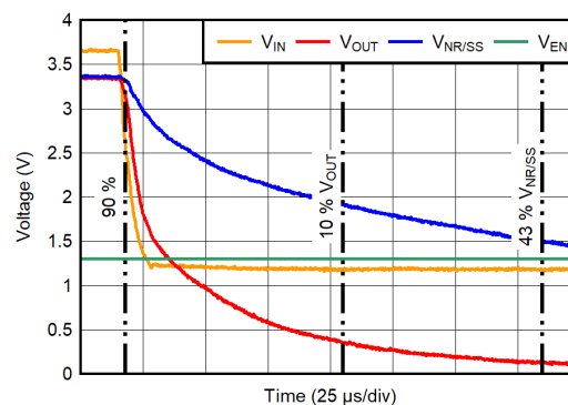
Figure 6-26. Shutdown Waveform for UVLO_{(IN)}
