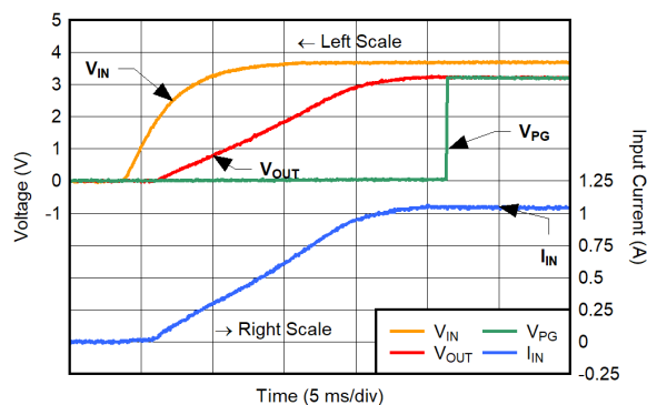
Figure 6-25. Start-Up Waveform for I_{OUT} = 1\text{ A}
