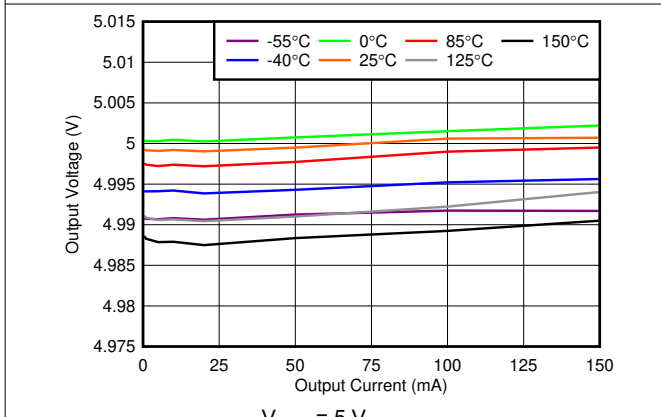
Figure 6-5. Load Regulation vs I_{OUT}
