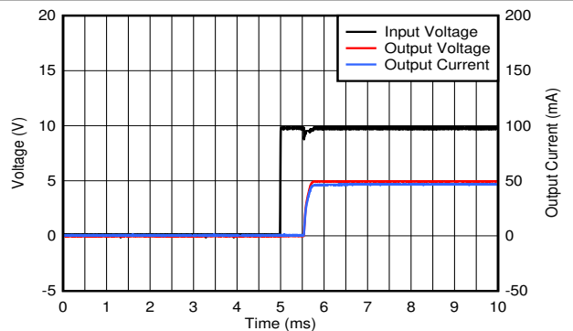
C_{OUT} = 10\ \mu\text{F} 6-30. Startup Plot
