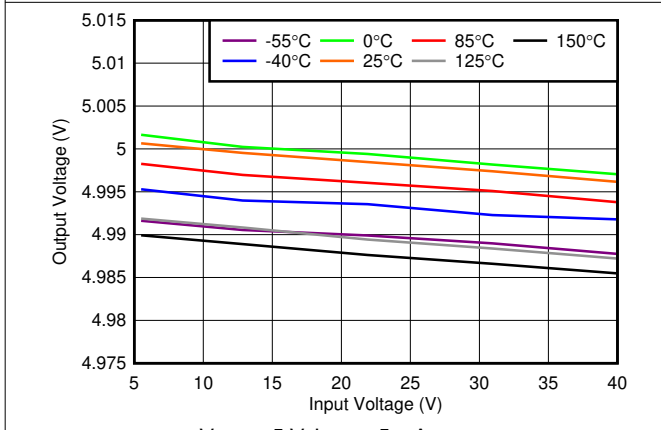
Figure 6-3. Line Regulation vs V_{IN}
