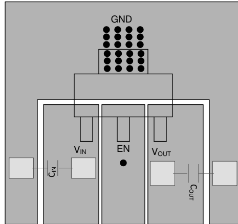
10-1. SOT-223 (DCY) Layout
