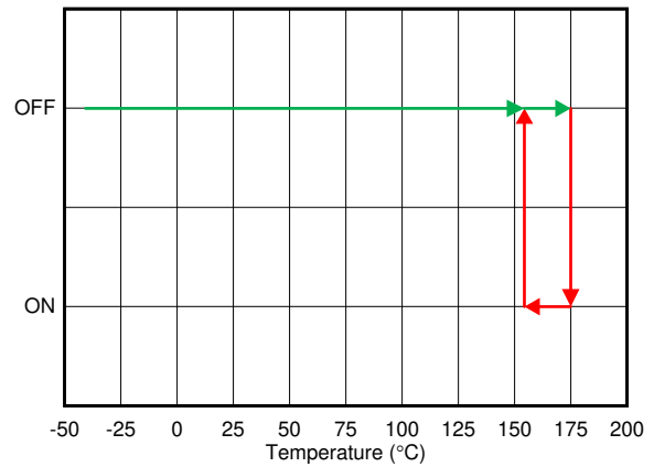
6-32. Thermal Shutdown
