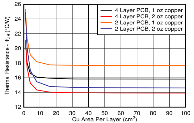
8-3. \psi_{JB} vs Copper Area 2s2p DRB Package
