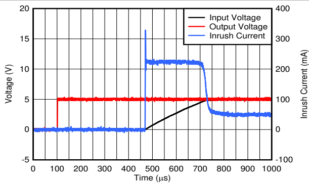
V_{IN} = 13.5\ \text{V} , C_{OUT} = 10\ \mu\text{F} 6-29. Startup Plot With EN
