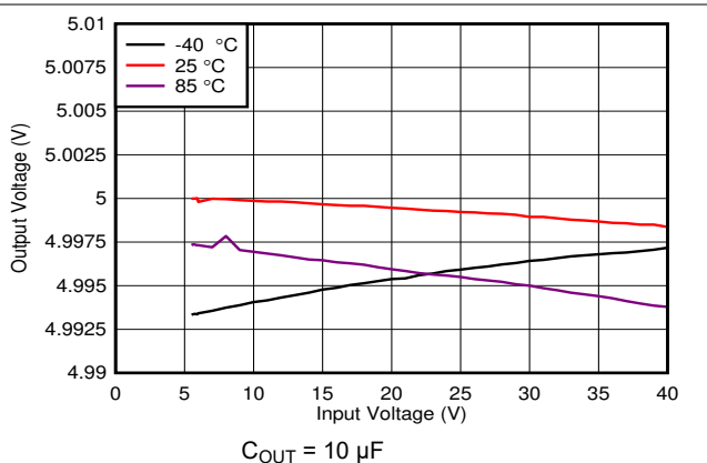
Figure 6-6. Line Regulation at 50 mA
