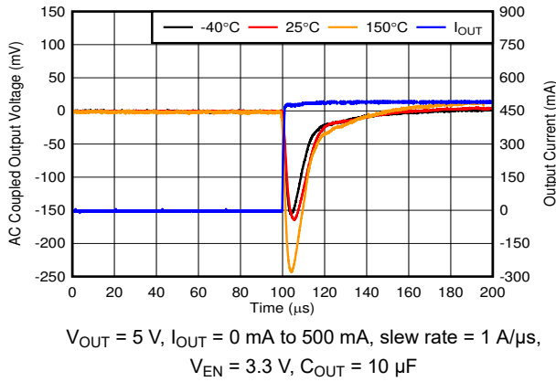
6-25. Load Transient, No Load to 500-mA Rising Edge
