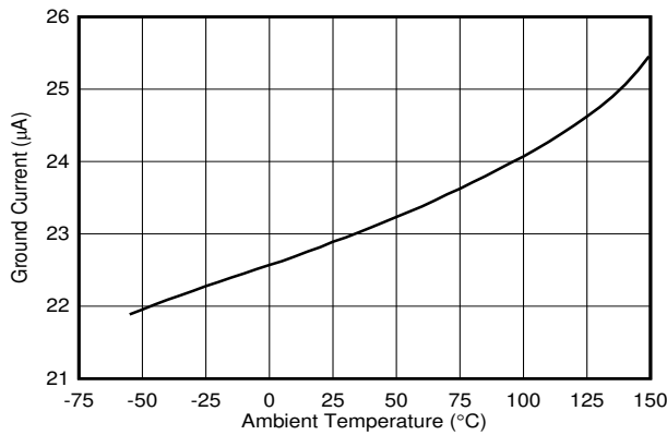
6-31. Ground Current at 500 \mu\text{A}
