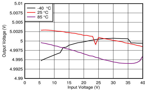
6-7. Line Regulation at 100 mA
