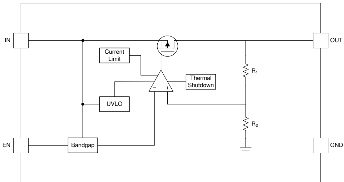
7-1. TPS7B86-Q1 Fixed Output Without PG
