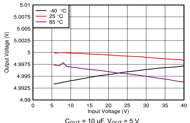
C_{OUT} = 10\ \mu\text{F} , V_{OUT} = 5\ \text{V} 6-6. Line Regulation at 50 mA
