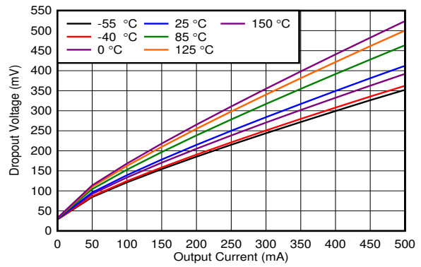
6-8. Dropout Voltage ( V_{DO} ) vs I_{OUT}
