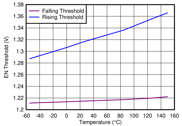
6-32. EN Threshold vs Temperature
