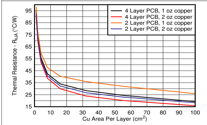
8-4. R_{\theta JA} vs Copper Area (KVU Package)
