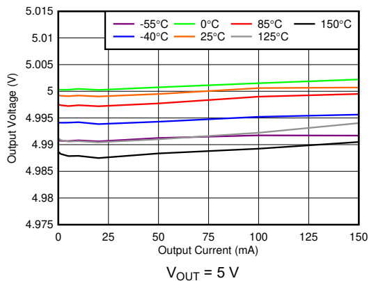
V_{OUT} = 5\ \text{V} 6-5. Load Regulation vs I_{OUT}
