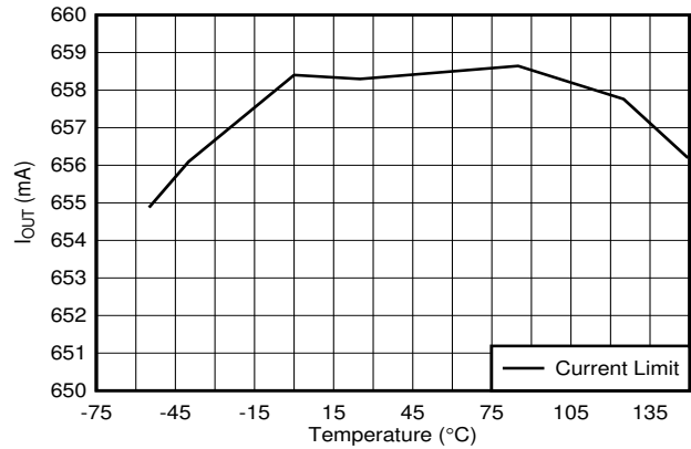
6-26. Output Current Limit vs Temperature
