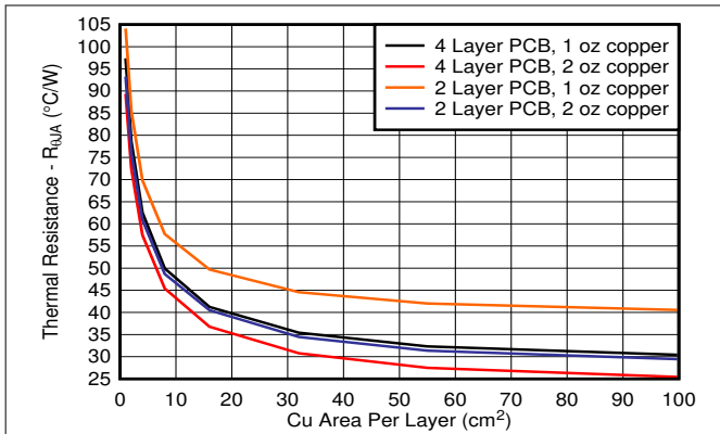
8-2. R_{\theta JA} vs Copper Area (DDA Package)
