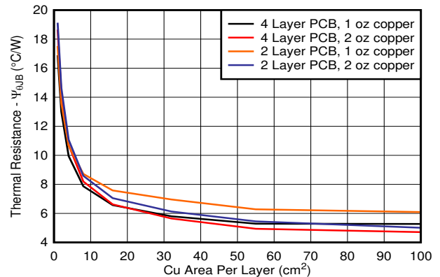
8-5. \psi_{JB} vs Copper Area (KVU Package)
