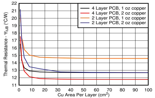
8-3. \psi_{JB} vs Copper Area (DDA Package)
