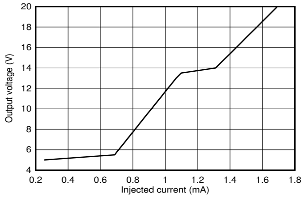
6-37. Output Voltage vs Injected Current
