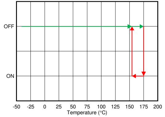
6-38. Thermal Shutdown
