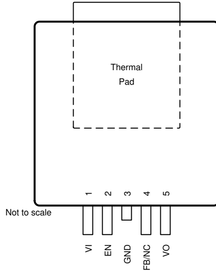
5-1. KVV Package, 5-Pin TO-252 (Top View)
