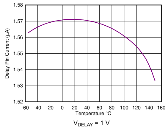
6-36. Delay Pin Current vs Temperature
