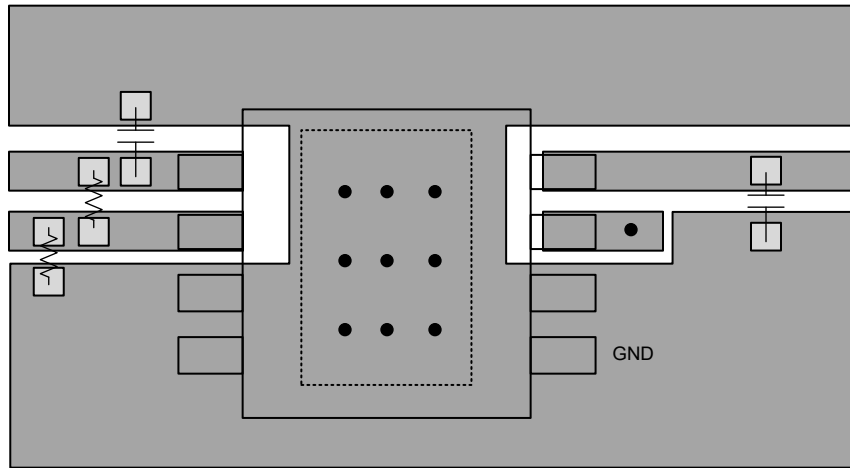
8-11. DDA Package Adjustable Output
