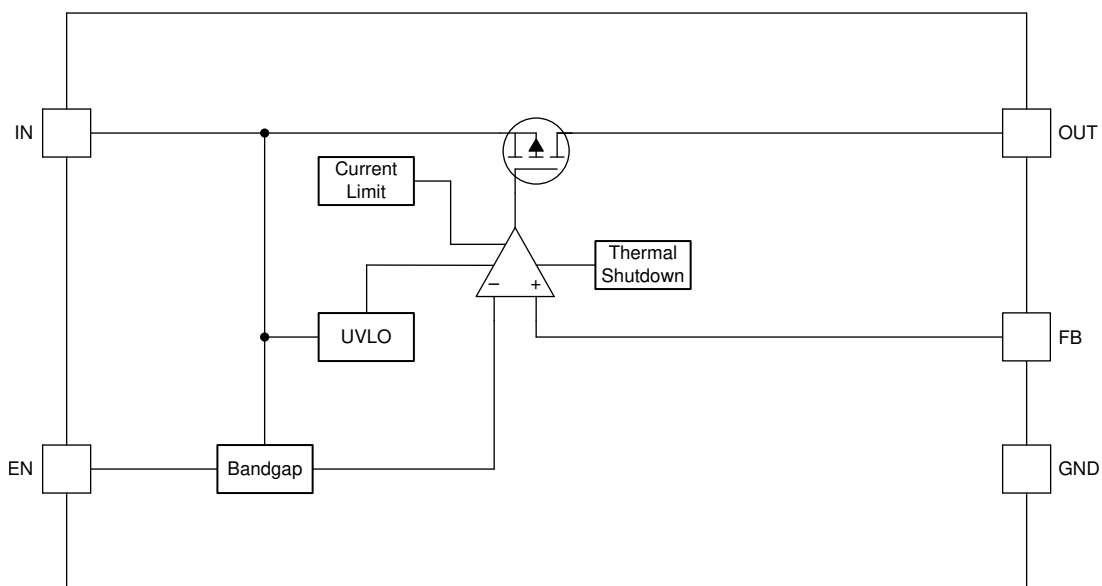
7-2. TPS7B86-Q1 Adjustable Output Without PG
