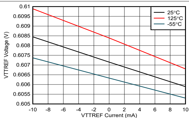
Figure 6-8. VTTREF Voltage vs VTTREF Current
