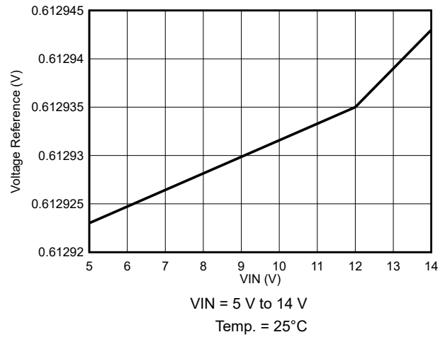
図 7-14. Voltage Reference Variation
