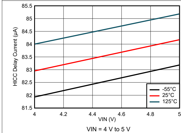
7-27. Hiccup Delay Current Variation
