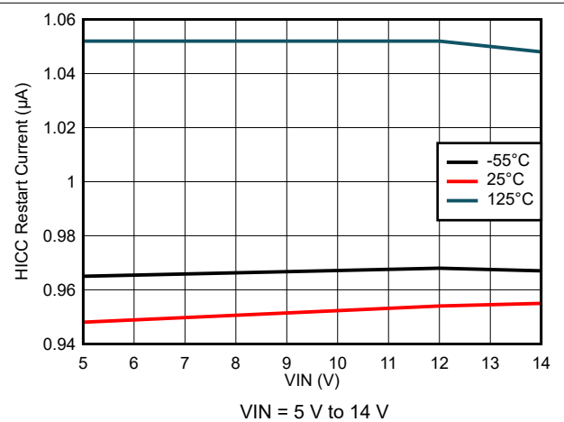
7-30. Hiccup Restart Current Variation
