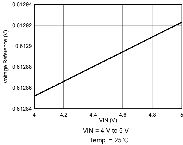
図 7-13. Voltage Reference Variation
