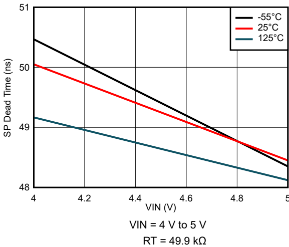
7-51. SP Dead Time Variation
