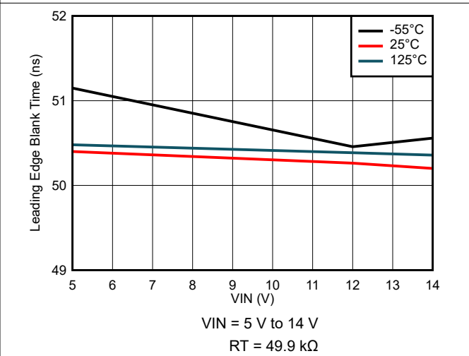
7-36. Leading Edge Blank Time Variation
