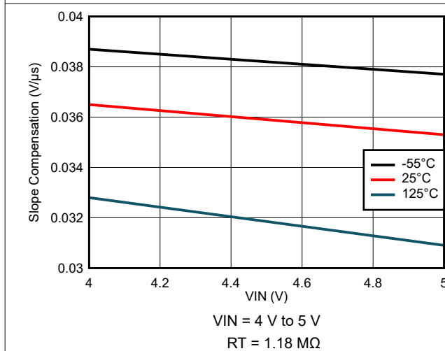
図 7-65. Slope Compensation Variation
