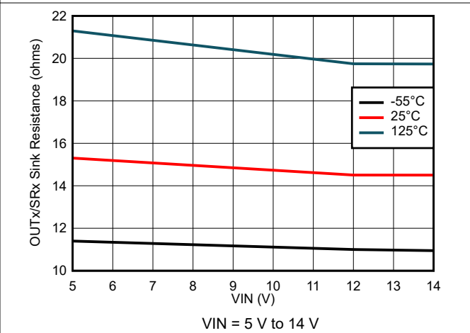
図 7-64. Output Sink Resistance Variation
