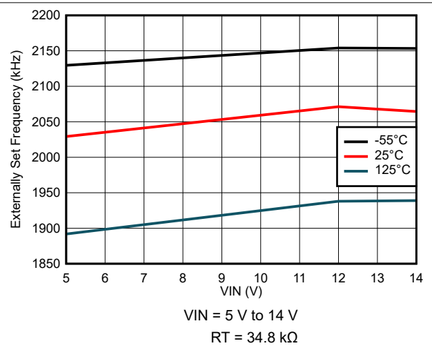
7-26. Externally Set Frequency Variation
