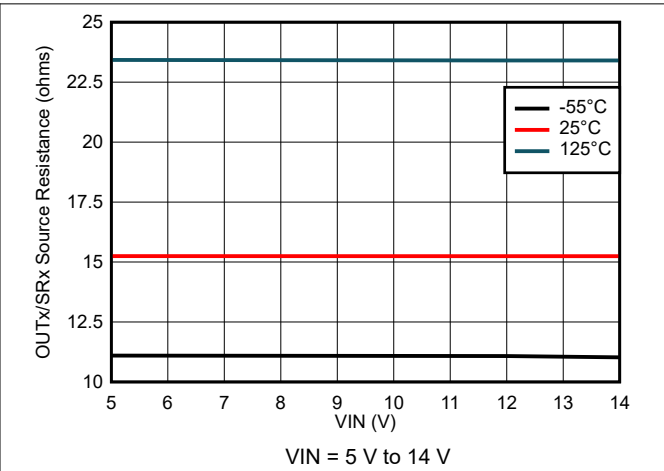
図 7-62. Output Source Resistance Variation
