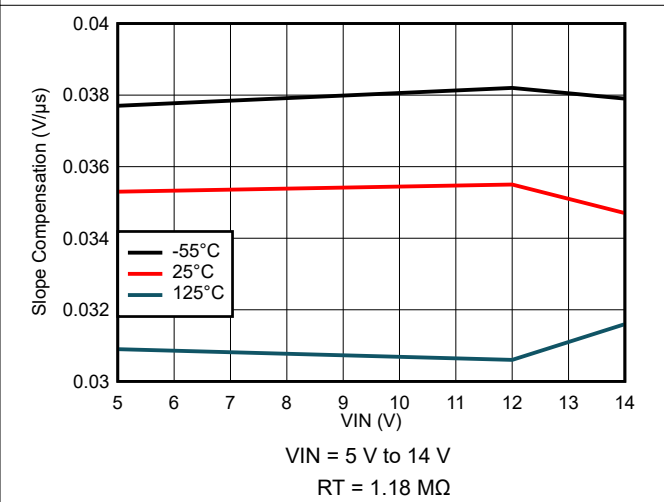
図 7-66. Slope Compensation Variation
