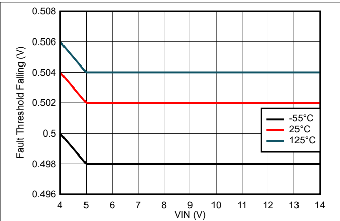
7-32. FAULT Threshold Falling Variation
