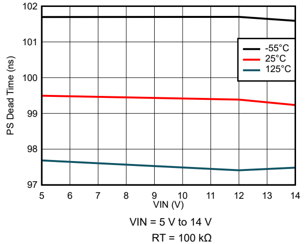
7-46. PS Dead Time Variation
