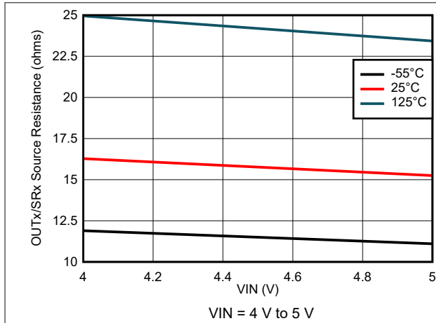
図 7-61. Output Source Resistance Variation
