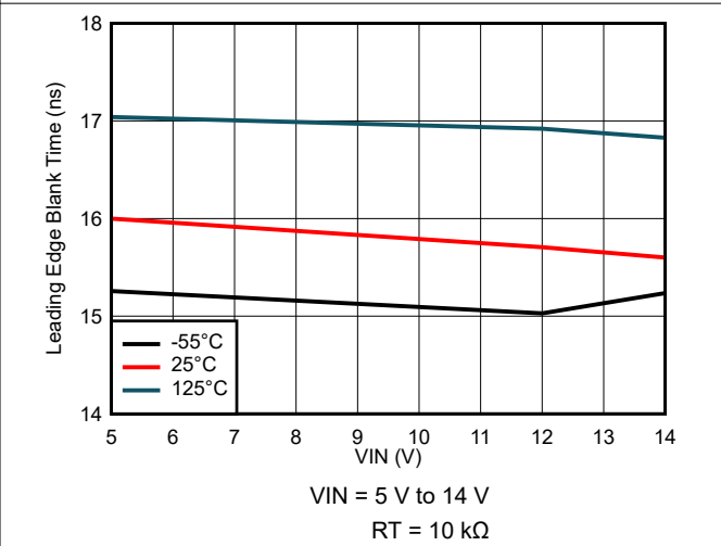
7-34. Leading Edge Blank Time Variation
