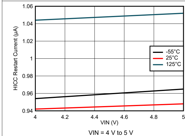
7-29. Hiccup Restart Current Variation
