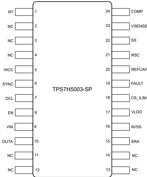
6-7. TPS7H5003-SP PW Package 24-Pin TSSOP (Top View)
