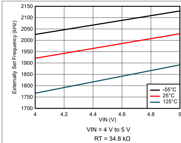
7-25. Externally Set Frequency Variation
