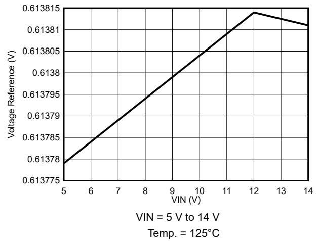
図 7-16. Voltage Reference Variation
