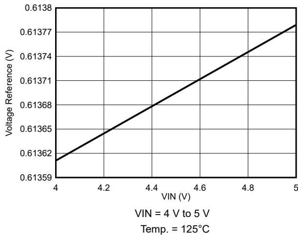
図 7-15. Voltage Reference Variation
