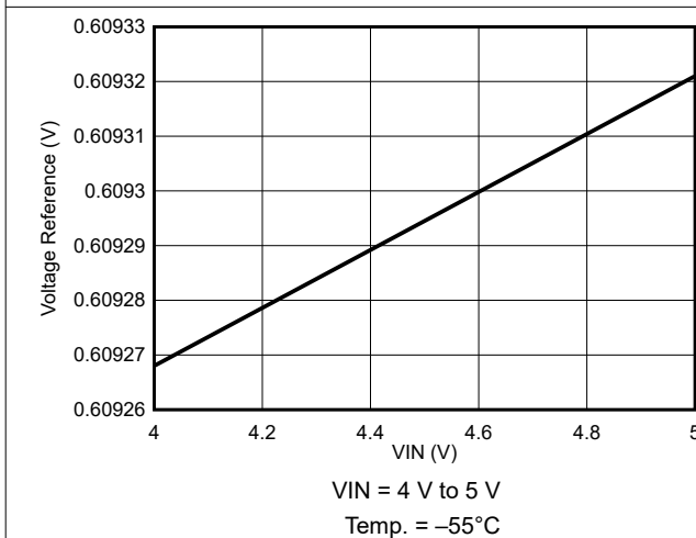
7-11. Voltage Reference Variation
