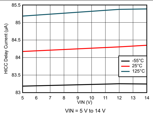
7-28. Hiccup Delay Current Variation
