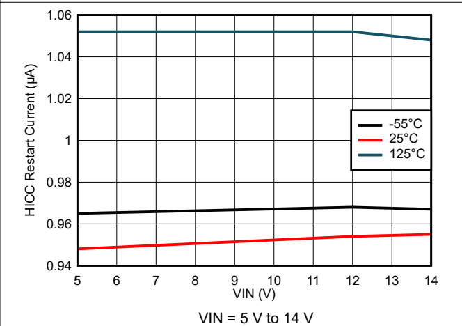
7-30. Hiccup Restart Current Variation
