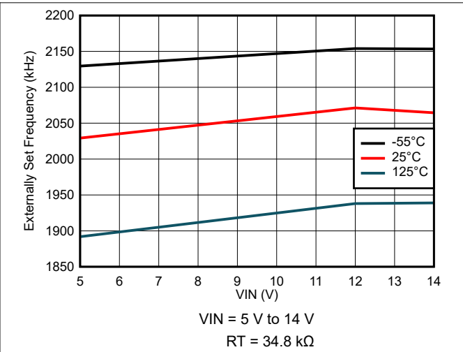
7-26. Externally Set Frequency Variation
