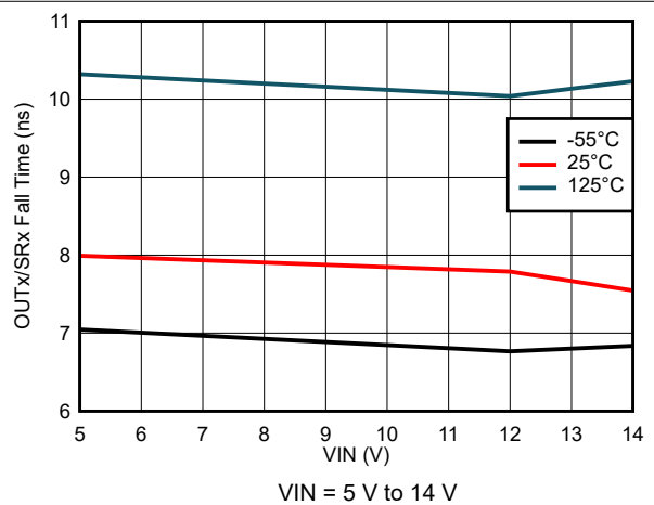
7-60. Output Fall Time Variation
