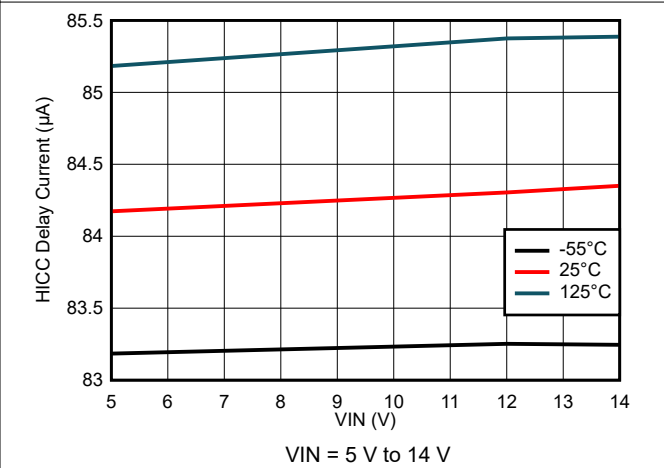
7-28. Hiccup Delay Current Variation
