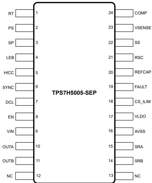
6-1. TPS7H5005-SEP PW Package 24-Pin TSSOP (Top View)
