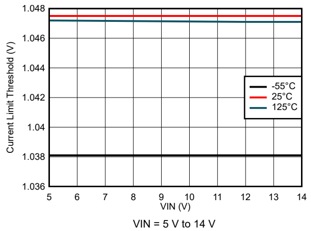
7-18. Current Limit Threshold Variation
