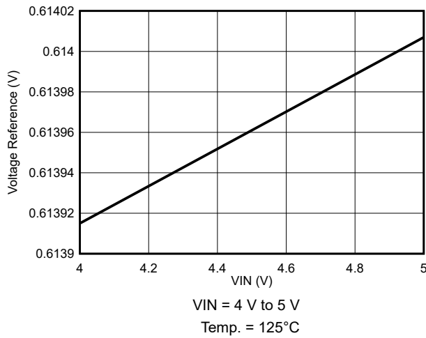
7-15. Voltage Reference Variation
