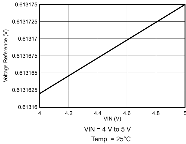
7-13. Voltage Reference Variation
