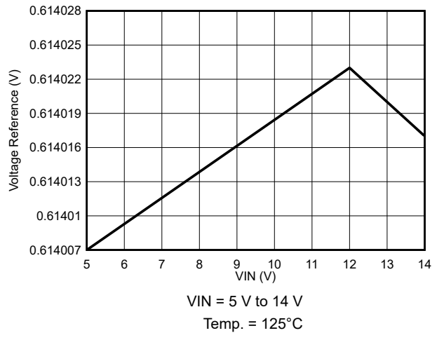
7-16. Voltage Reference Variation
