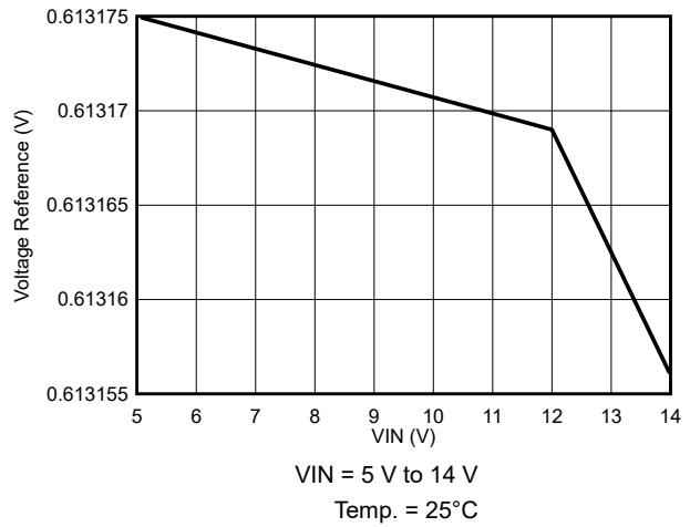
7-14. Voltage Reference Variation
