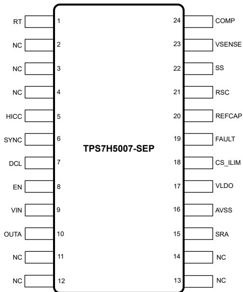
6-3. TPS7H5007-SEP PW Package 24-Pin TSSOP (Top View)
