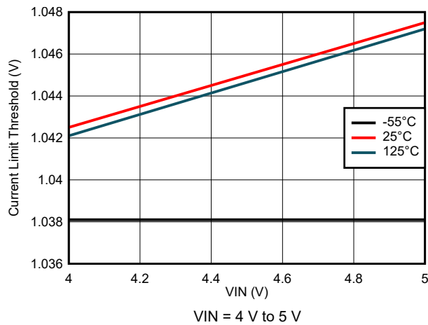
7-17. Current Limit Threshold Variation
