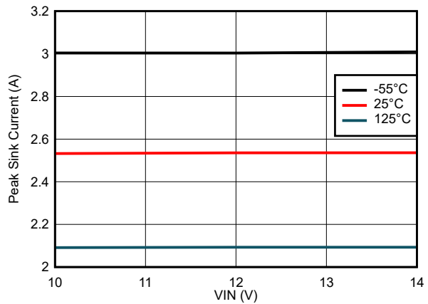
7-10. Peak Sink Current vs VIN Voltage
