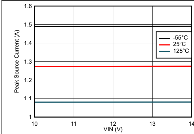
7-9. Peak Source Current vs VIN Voltage
