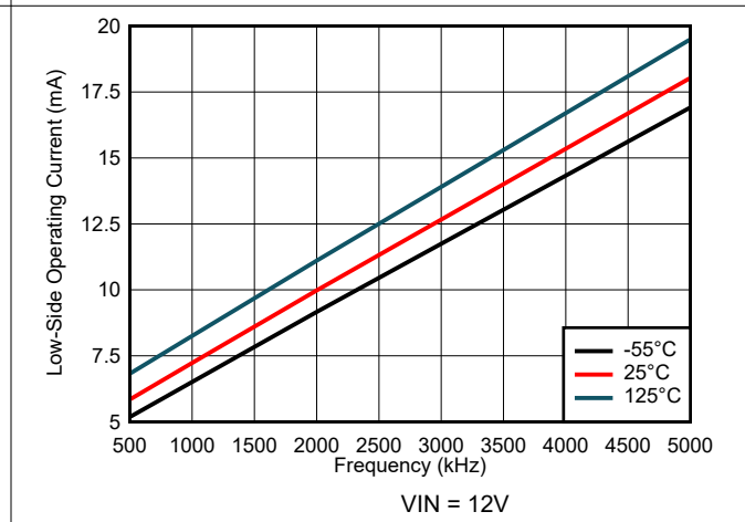
7-42. Low-Side Operating Current vs Frequency (IIM)
