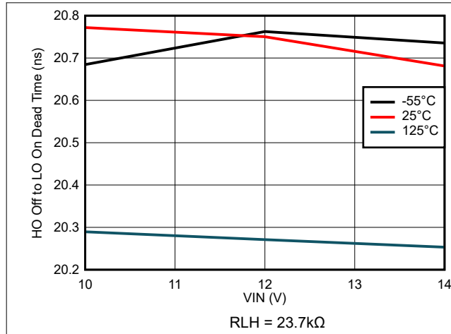
7-37. HO Off to LO On Dead Time vs VIN Voltage
