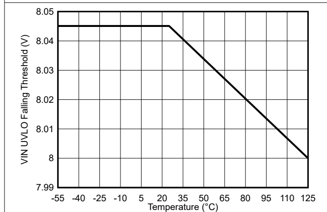
7-27. VIN UVLO Falling Threshold vs Temperature
