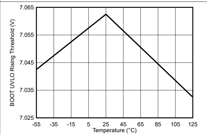
7-28. BOOT UVLO Rising Threshold vs Temperature
