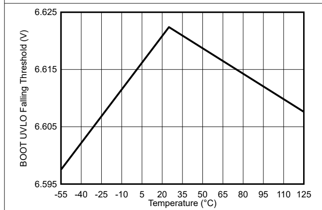
7-29. BOOT UVLO Falling Threshold vs Temperature
