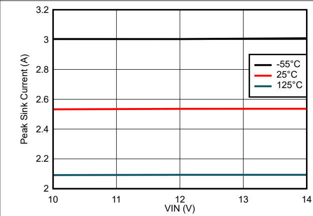
7-10. Peak Sink Current vs VIN Voltage
