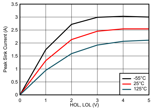
7-12. Peak Sink Current vs Output Voltage
