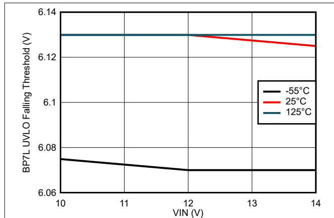
7-25. BP7L UVLO Falling Threshold vs VIN Voltage
