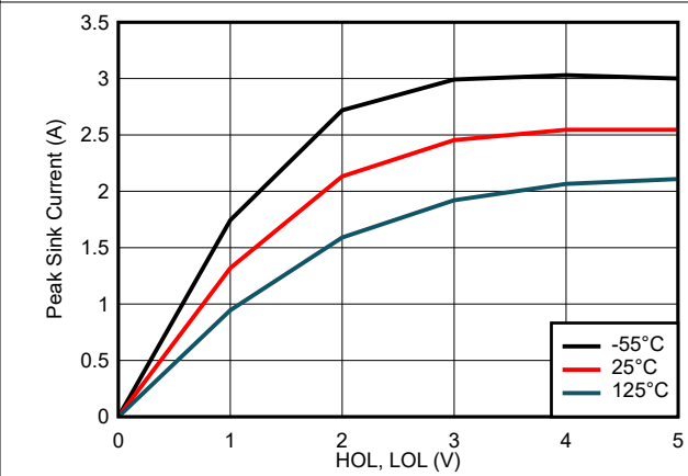
7-12. Peak Sink Current vs Output Voltage
