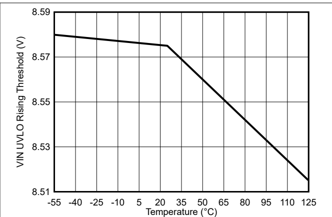
7-26. VIN UVLO Rising Threshold vs Temperature
