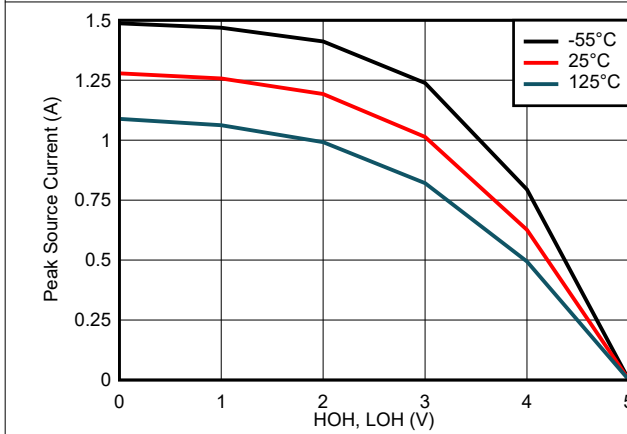
7-11. Peak Source Current vs Output Voltage
