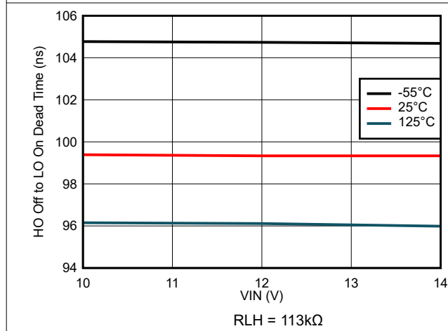
7-39. HO Off to LO On Dead Time vs VIN Voltage
