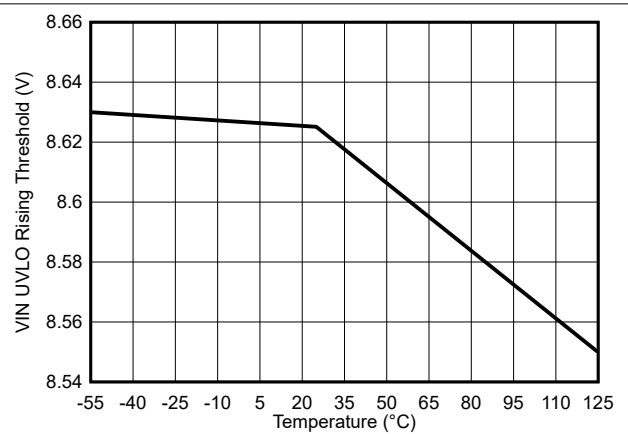
7-26. VIN UVLO Rising Threshold vs Temperature
