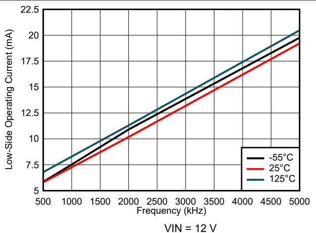
7-42. Low-Side Operating Current vs Frequency (IIM)
