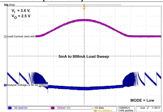
Figure 39. TPS826951 AC Load Transient Response
