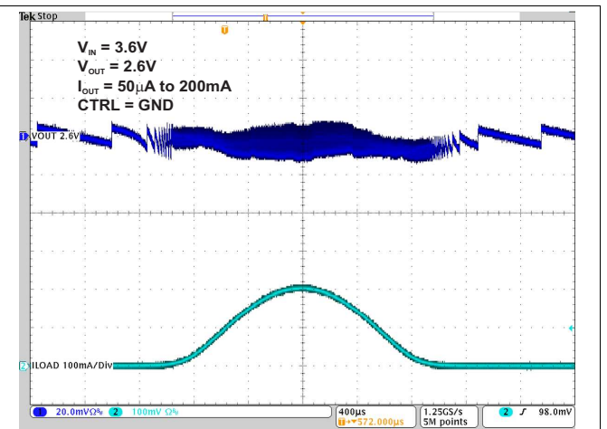
Figure 33. TPS82740B AC Load Sweep V_{OUT} = 2.6V
