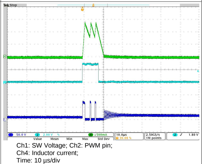
Figure 39. PWM Dimming: 250Hz, 0.25% Duty Cycle
