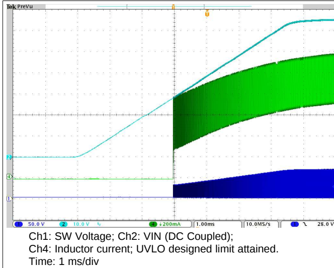
Figure 36. Startup Transient
