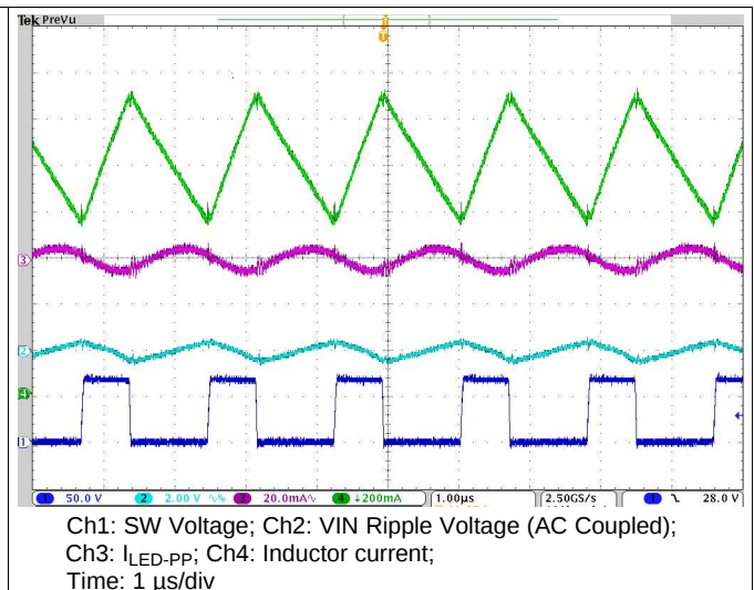
Figure 35. Normal Operation
