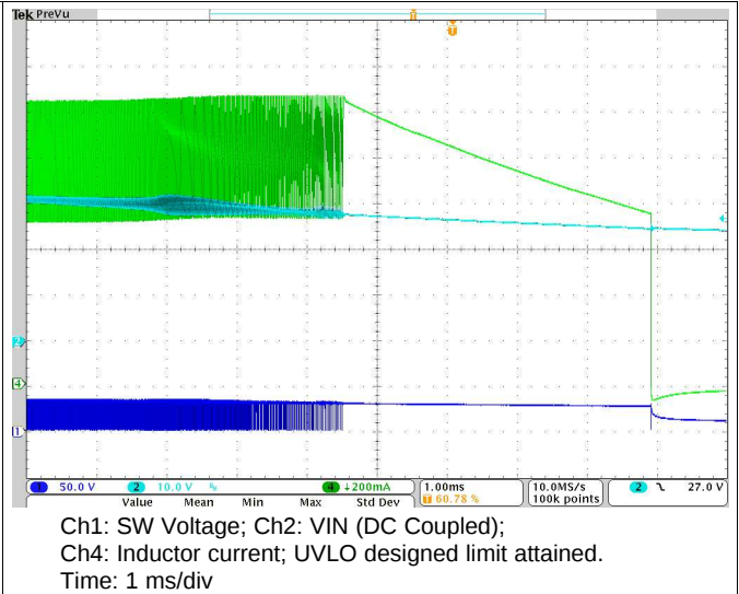
Figure 37. Shut-Down Transient
