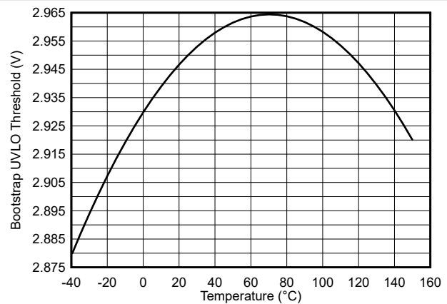
FIG 6-8. Bootstrap UVLO Threshold vs Temperature
