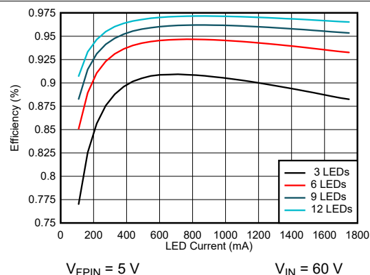
FIG 6-20. Efficiency vs LED Current
