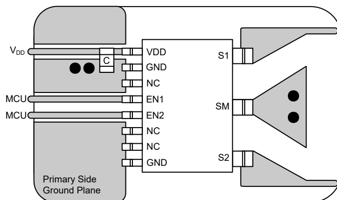
9-23. TPSI2072-Q1 Layout with Interlayer Stitch Capacitance: Top Layer (1)
