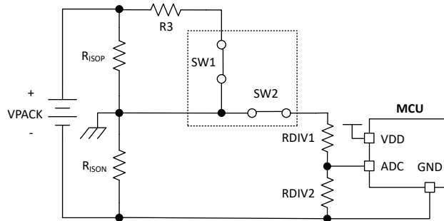
FIG 9-5. Battery V- Reference Switch Positions for ADC2 Measurement
