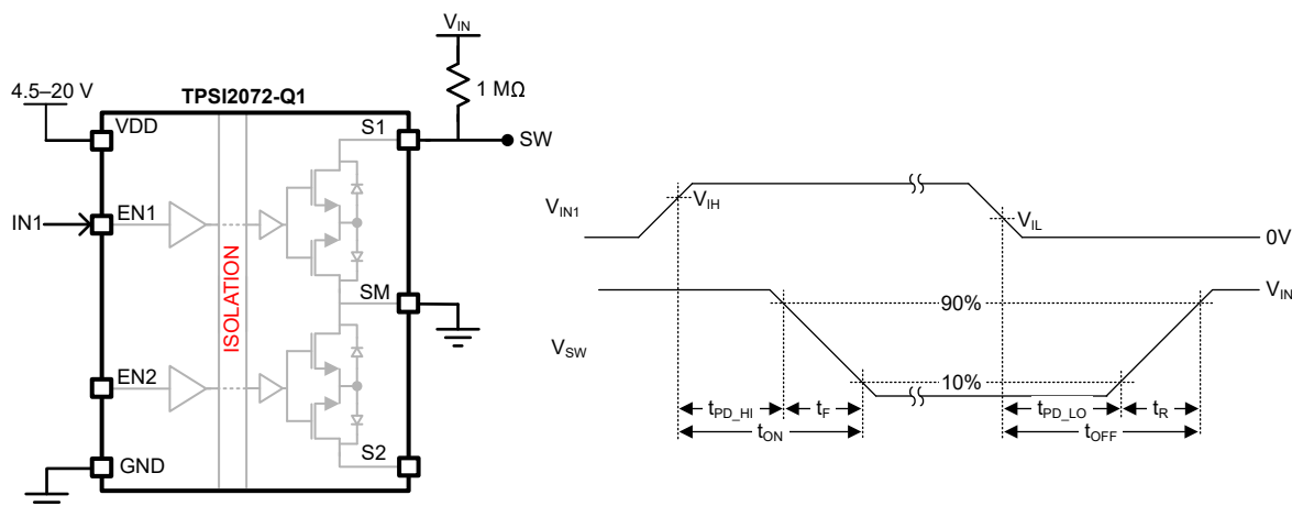
7-1. Timing Diagram, EN1 Switching
