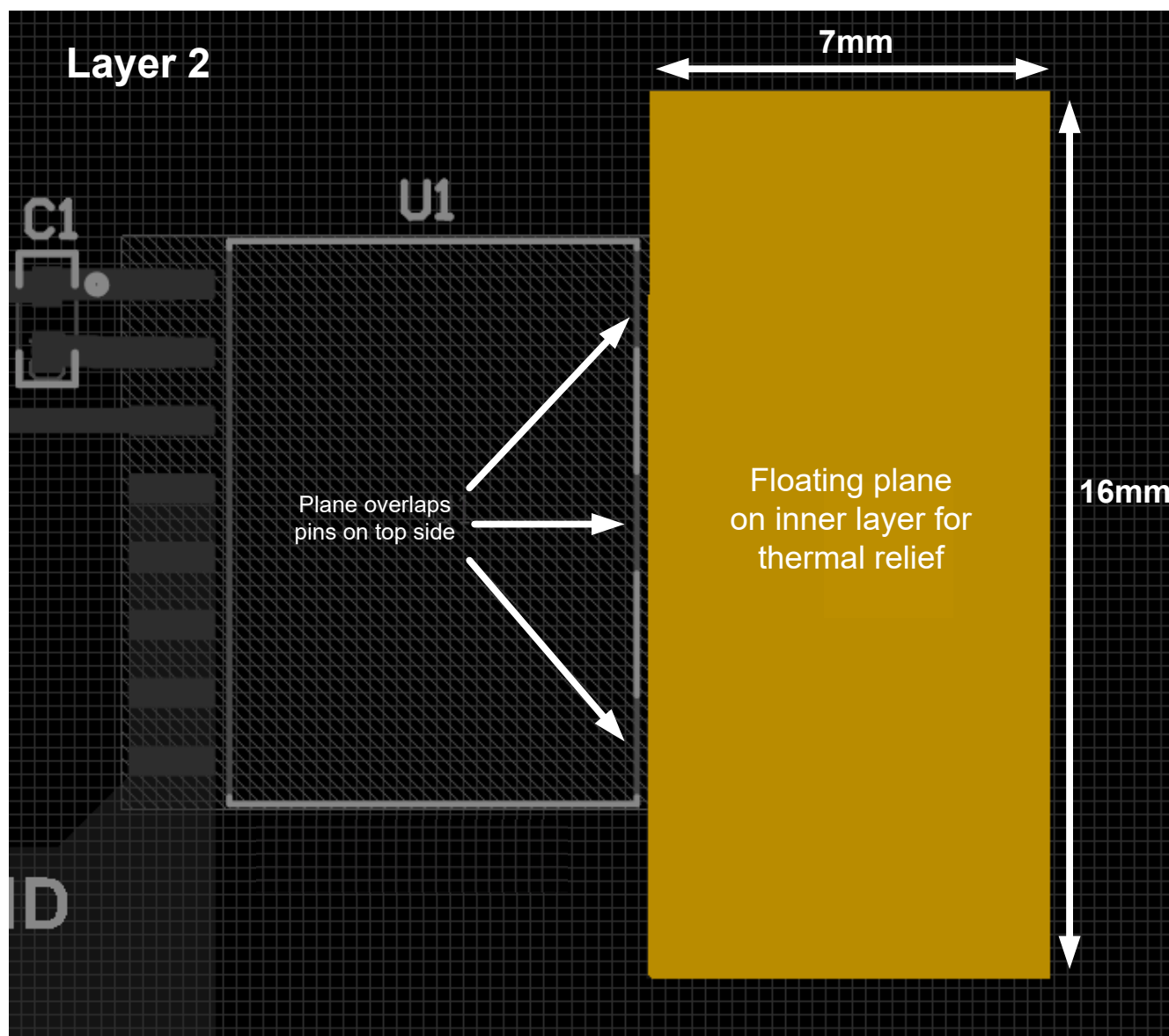
9-20. TPSI2072-Q1 Secondary Side Layout Recommendation for Optimized Thermal Performance: Inner Layer 2
