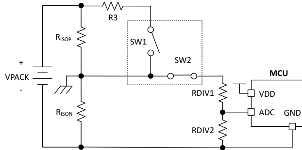
FIG 9-4. Battery V- Reference Switch Positions for ADC1 Measurement
