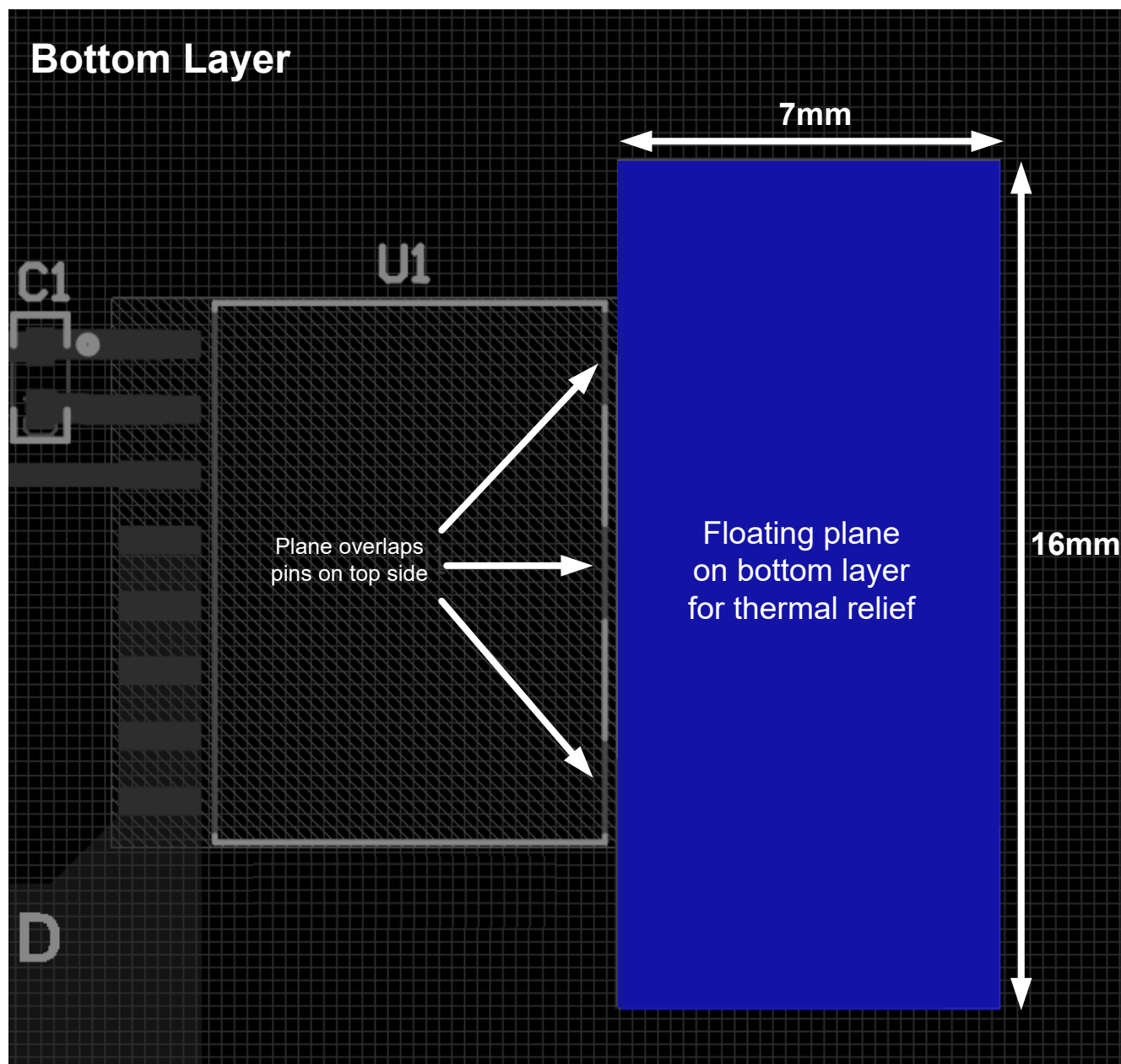
9-22. TPSI2072-Q1 Secondary Side Layout Recommendation for Optimized Thermal Performance: Bottom Layer 4
