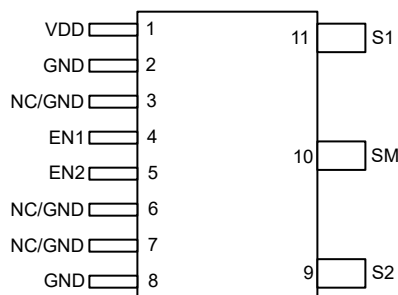
FIG 5-1. TPSI2072-Q1 DWQ Package, 11-Pin SOIC (Top View)
