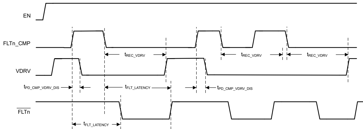
图 7-3. VDRV Auto-Recovery Timing (CE = 1 or CE = VDDP)
