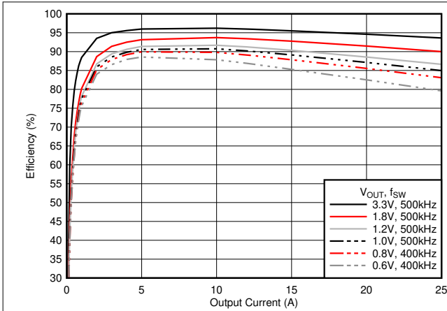
6-8. Efficiency vs Output Current
