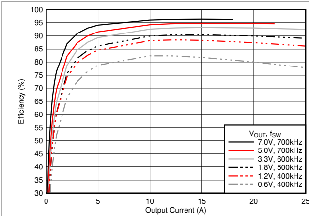
6-1. Efficiency vs Output Current
