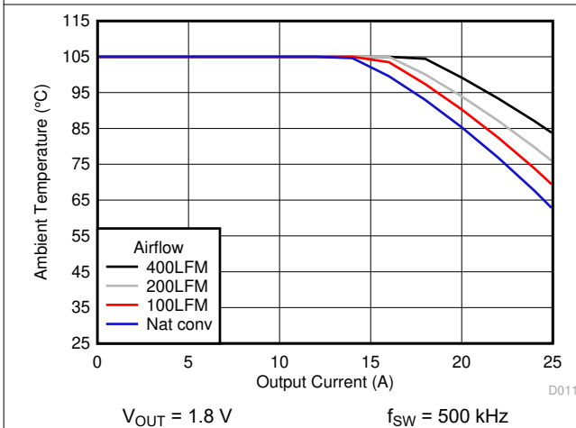
6-12. Safe Operating Area
