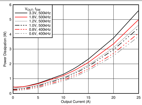
6-9. Power Dissipation vs Output Current
