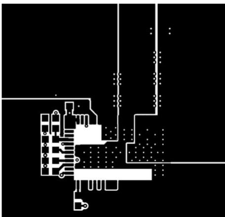
10-3 . Top-Layer Layout (Top View)
