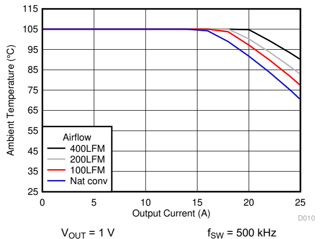
6-11. Safe Operating Area
