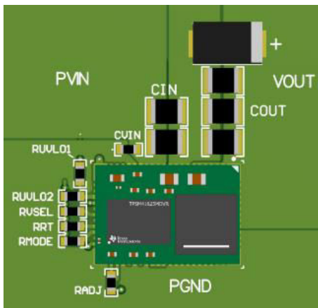
10-1 . Top-Layer Components (Top View)
