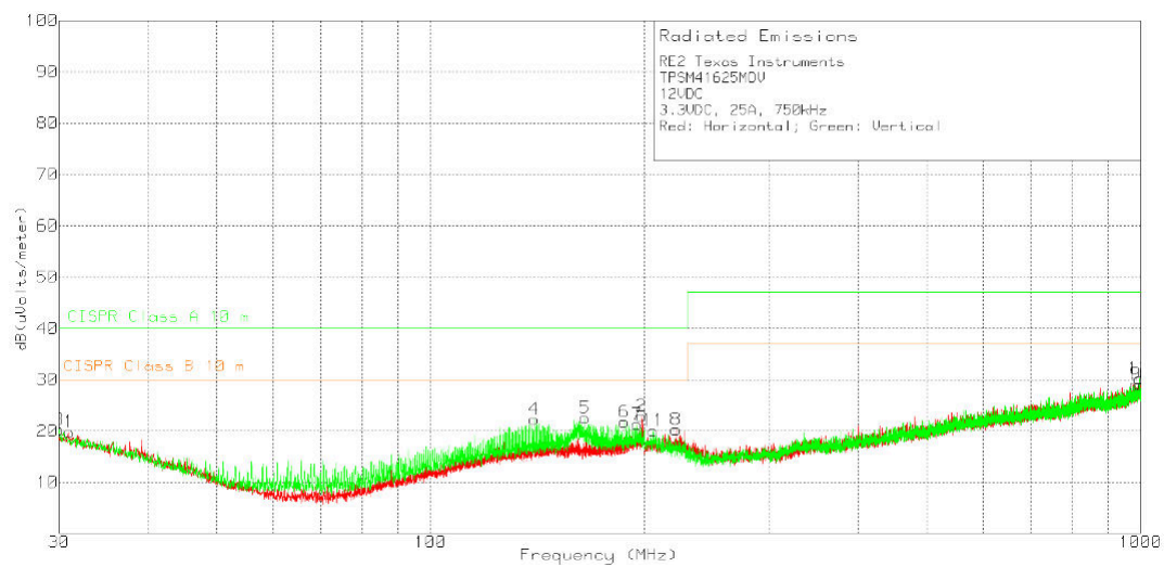
10-6. Radiated Emissions 12-V Input, 3.3-V Output, 25-A Load (EN55011 Class B)
