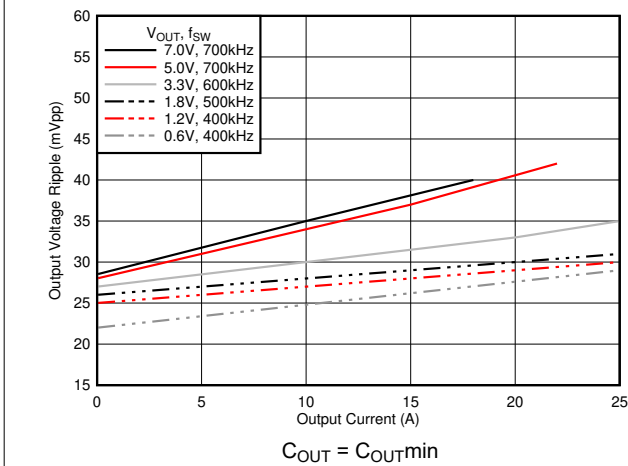
6-3. Output Voltage Ripple
