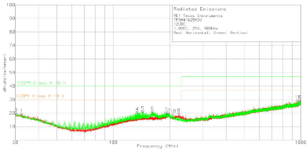
10-5. Radiated Emissions 12-V Input, 1.8-V Output, 25-A Load (EN55011 Class B)
