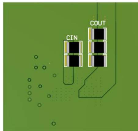
10-2 . Bottom-Layer Components (Top View)
