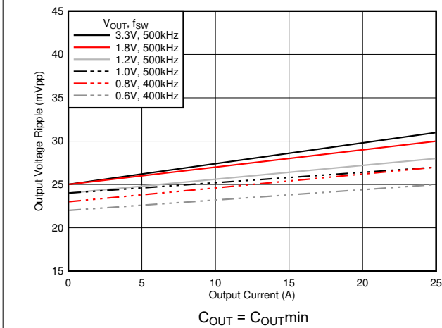
6-10. Output Voltage Ripple
