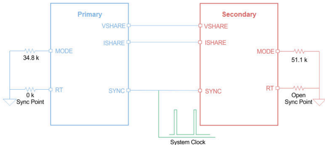
FIG 7-6. 2-Phase Stackable, 180° Phase Shift: Primary and Secondary Sync to External System Clock
