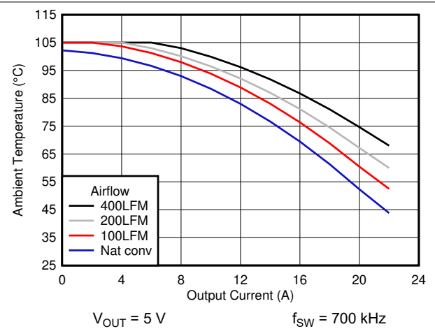
6-6. Safe Operating Area
