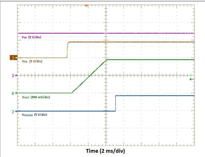
8-3. Start-Up Waveforms
