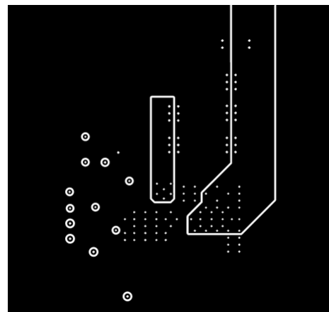
10-4 . Bottom-Layer Layout (Top View)
