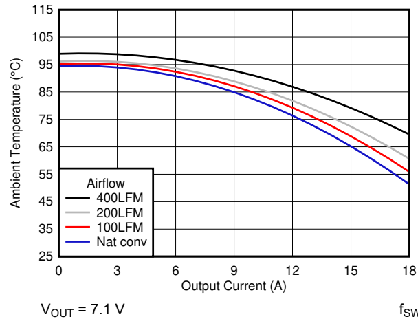
6-7. Safe Operating Area
