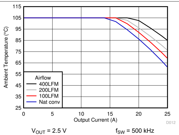
6-13. Safe Operating Area
