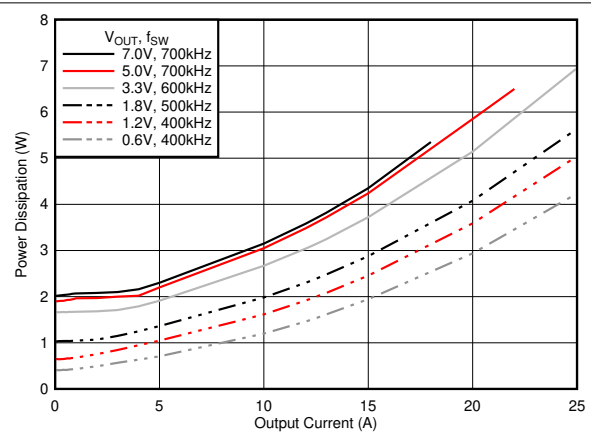
6-2. Power Dissipation vs Output Current
