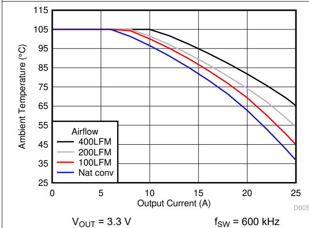
6-5. Safe Operating Area
