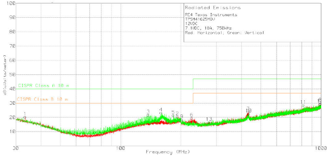
10-7. Radiated Emissions 12-V Input, 7.1-V Output, 18-A Load (EN55011 Class B)
