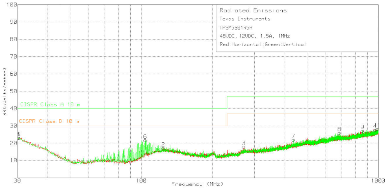
☒ 11-9. Radiated Emissions 48-V Input, 12-V Output, 1.5-A Load
