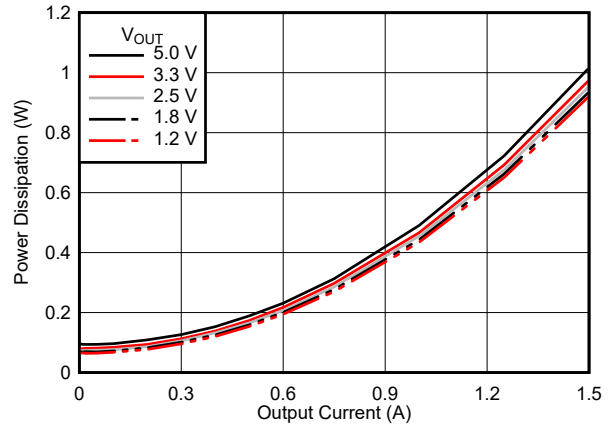
7-2. Power Dissipation
