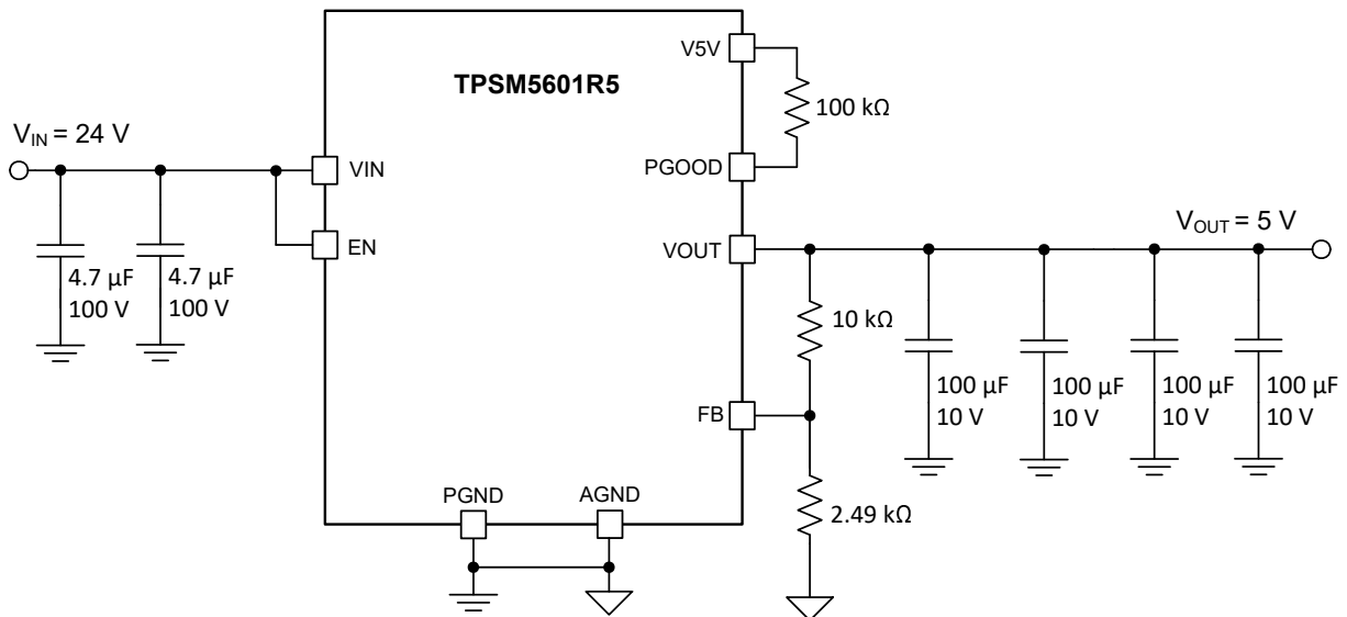
☒ 9-1. TPSM5601R5 Typical Schematic
