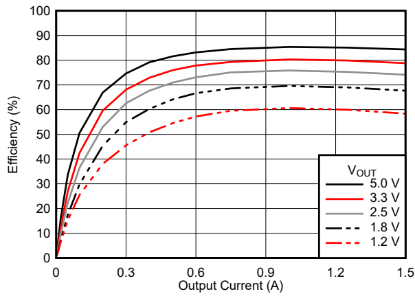
7-12. Efficiency
