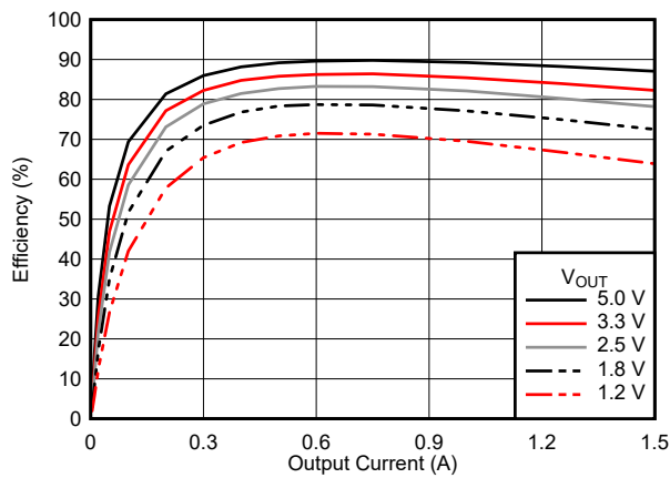
7-7. Efficiency
