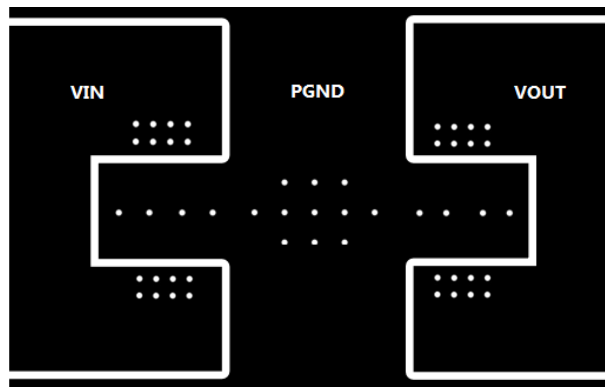
Fig 11-3. Typical Mid-Layer
