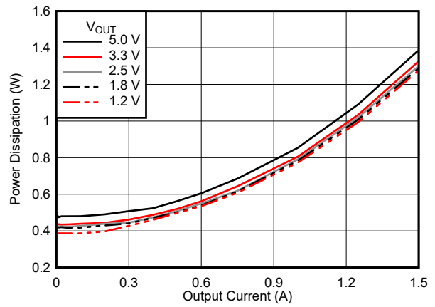
7-13. Power Dissipation
