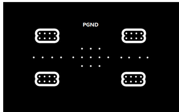
Fig 11-4. Typical PGND-Layer
