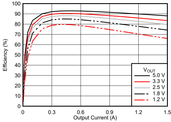
7-1. Efficiency
