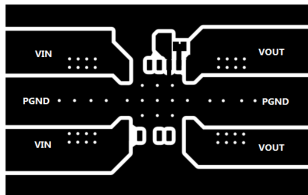
Fig 11-2. Typical Top-Layer
