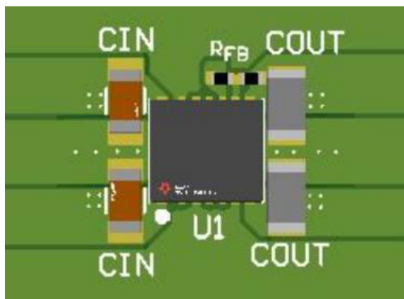
Fig 11-1. Typical Layout
