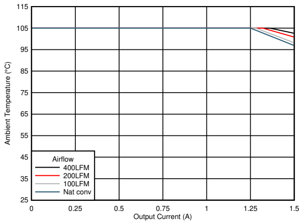
7-5. Safe Operating Area ( V_{OUT} = 3.3\text{ V} )
