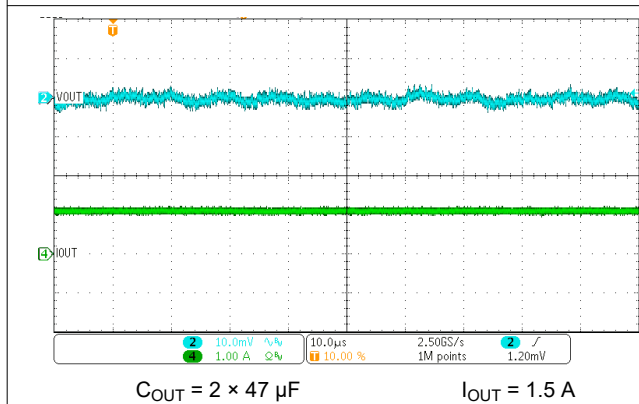
9-4. Output Ripple Waveform
