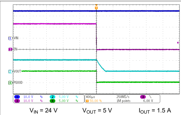
9-3. Enable Shutdown Waveforms
