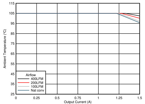
7-4. Safe Operating Area (V OUT = 1.2 V)
