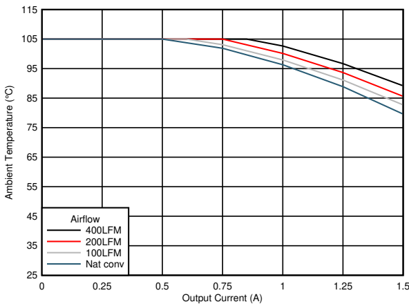
7-17. Safe Operating Area (V OUT = 12 V)
