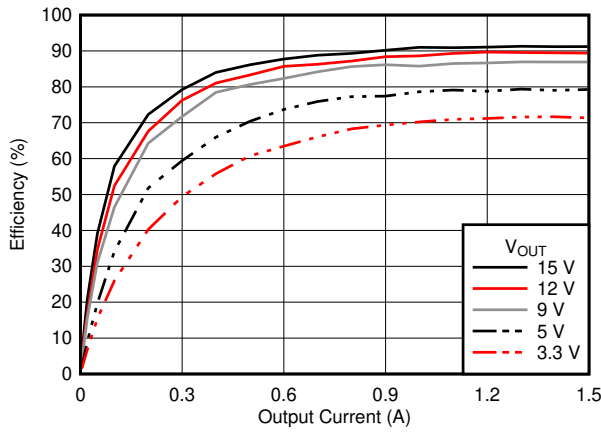
7-13. Efficiency
