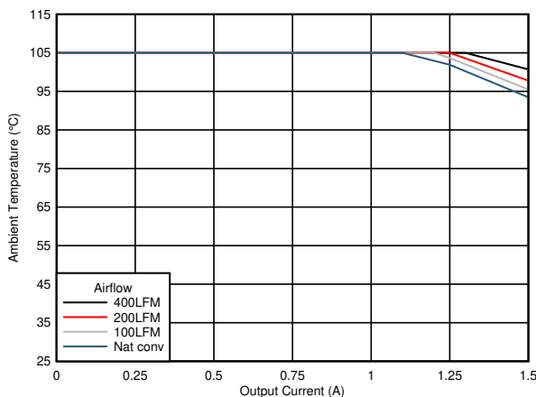
7-11. Safe Operating Area (V OUT = 5.0 V)
