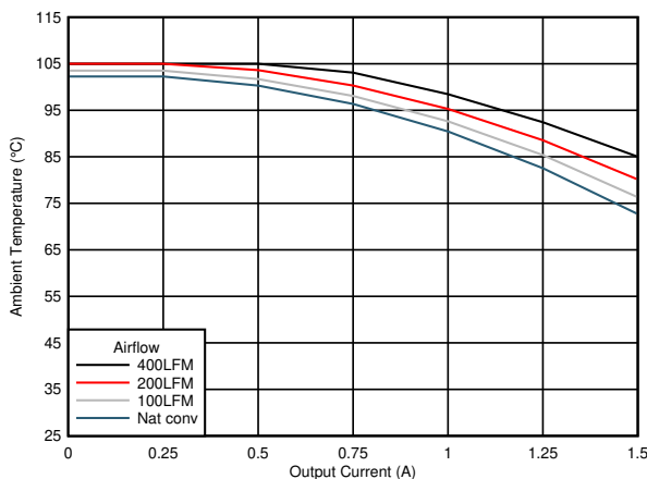
7-23. Safe Operating Area (V OUT = 12 V)
