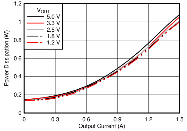
7-2. Power Dissipation
