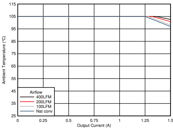
7-5. Safe Operating Area (V OUT = 3.3 V)
