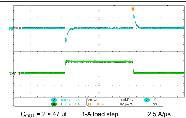
9-5. Transient Response Waveform
