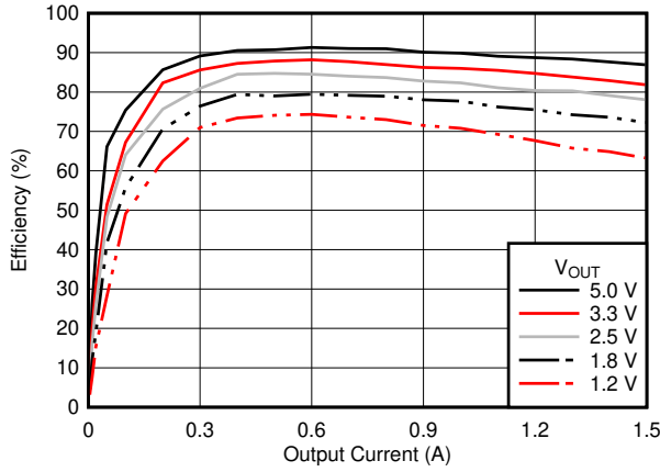
7-1. Efficiency
