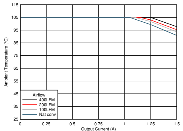
7-10. Safe Operating Area (V OUT = 1.8 V)
