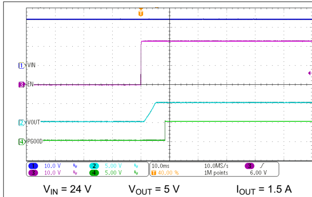
9-2. Start-up Waveforms
