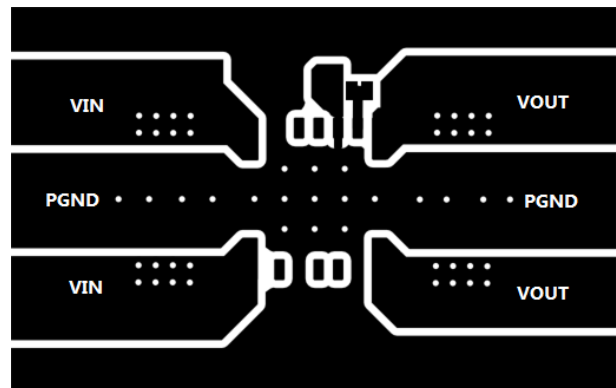
Figure 11-2. Typical Top-Layer
