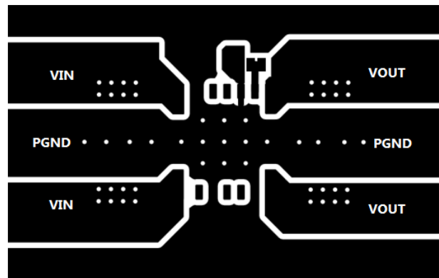
10-2. Typical Top-Layer
