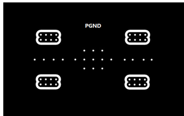
10-4. Typical PGND-Layer
