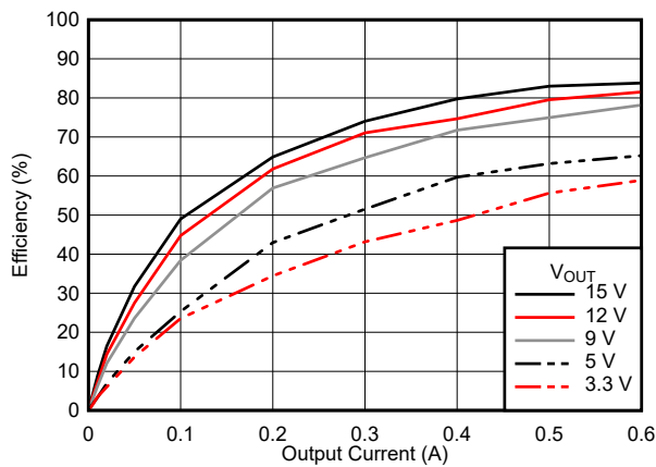
6-15. Efficiency
