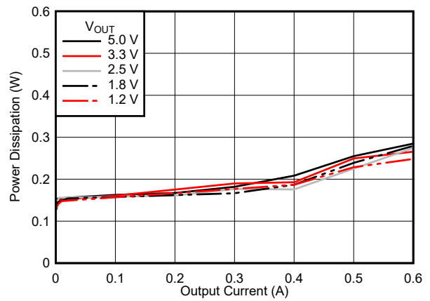
6-2. Power Dissipation
