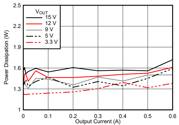
6-16. Power Dissipation
