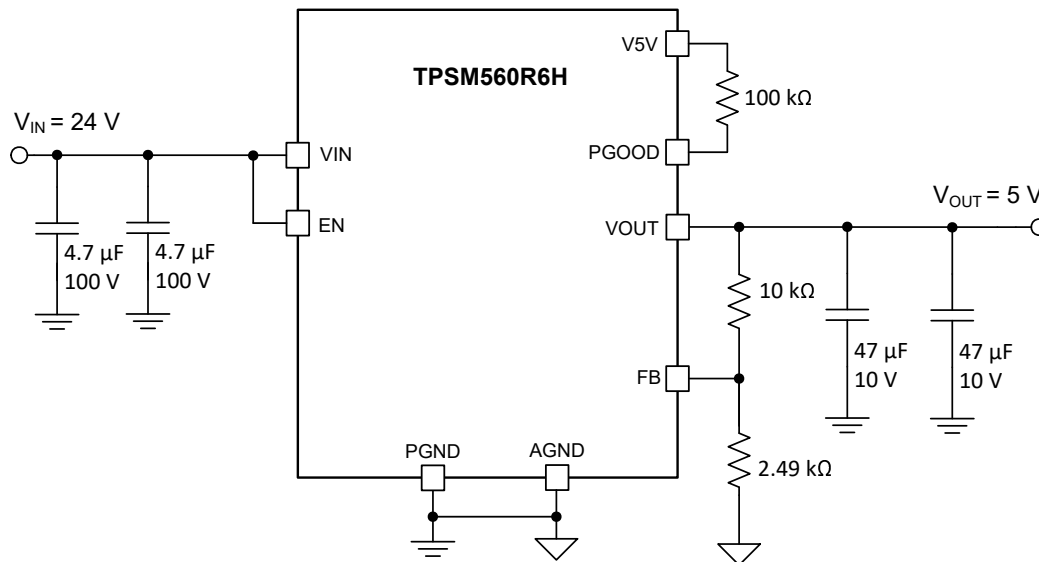
☒ 8-1. TPSM560R6H Typical Schematic
