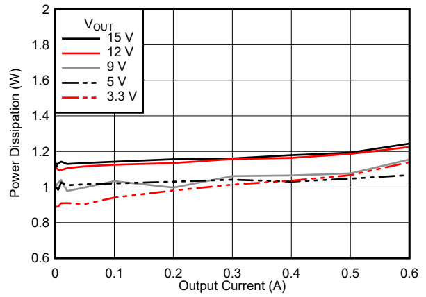
6-10. Power Dissipation
