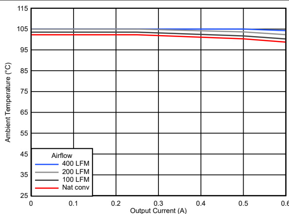
6-19. Safe Operating Area ( V_{OUT} = 12\text{ V} )
