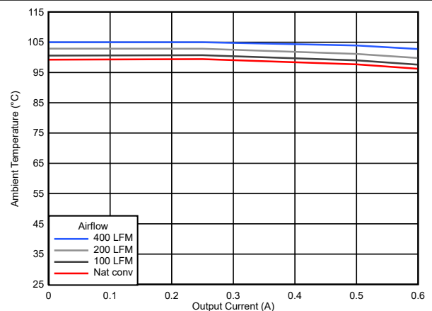
6-18. Safe Operating Area ( V_{OUT} = 5.0\text{ V} )
