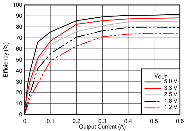
6-1. Efficiency
