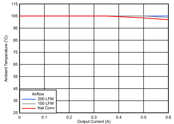
6-12. Safe Operating Area ( V_{OUT} < 10\text{ V} )
