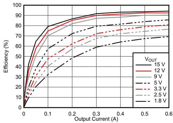
6-5. Efficiency
