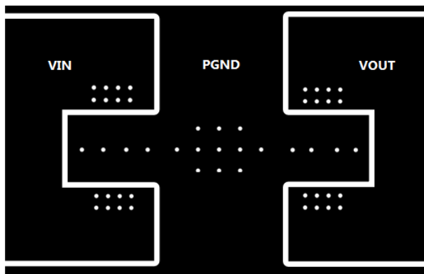
10-3. Typical Mid-Layer
