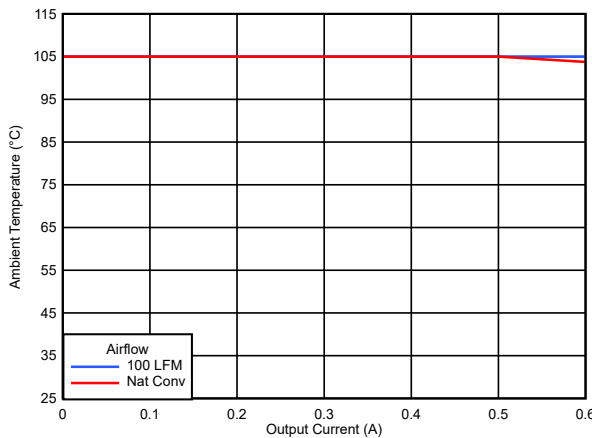
6-13. Safe Operating Area ( V_{OUT} = 12\text{ V} )
