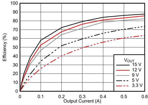
6-9. Efficiency
