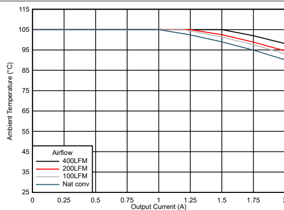
7-16. Safe Operating Area ( V_{OUT} = 12\text{ V} )
