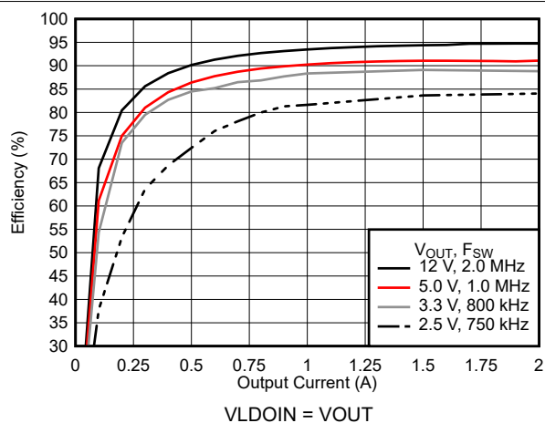
7-11. Efficiency
