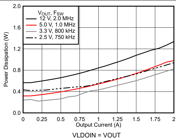
7-12. Power Dissipation
