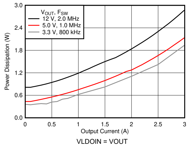
図 7-20. Power Dissipation
