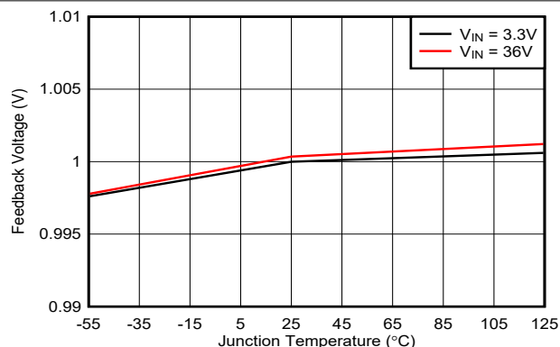
Figure 7-2. Feedback Voltage
