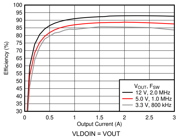
図 7-19. Efficiency
