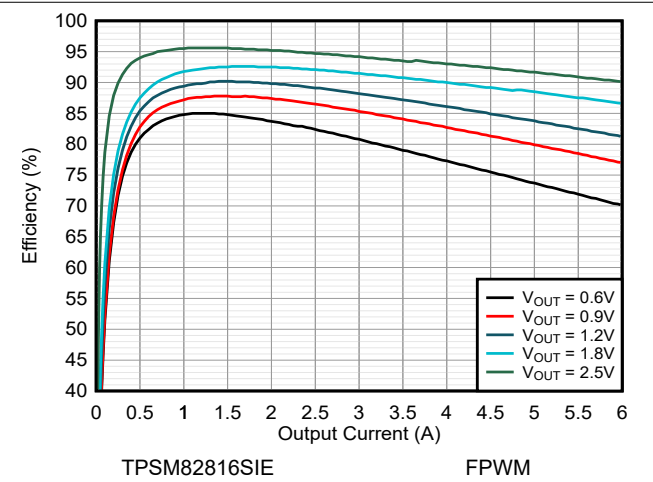
8-11. Efficiency V_{IN} = 3.3\text{ V} and T_A = 85^\circ\text{C}
