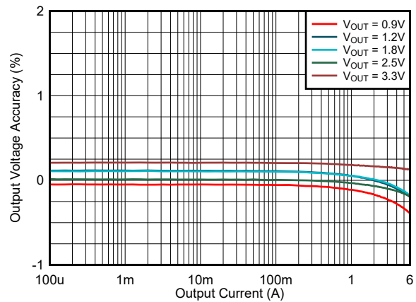
8-15. Load Regulation V IN = 5.0 V (FPWM)
