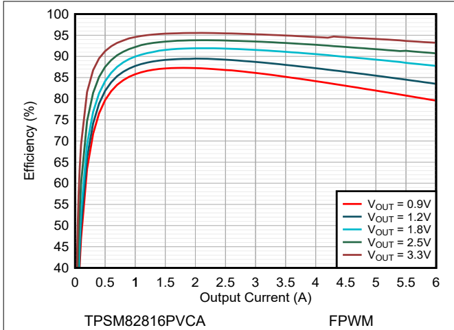
8-8. Efficiency V_{IN} = 5.0\text{ V} and T_A = 85^\circ\text{C}
