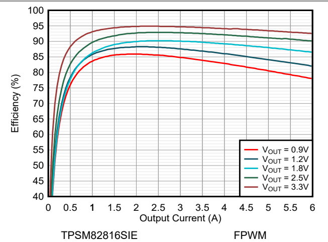
8-9. Efficiency V_{IN} = 5.0\text{ V} and T_A = 85^\circ\text{C}
