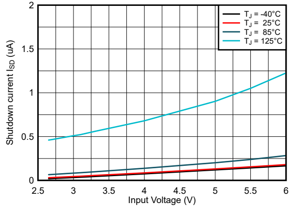
Figure 6-2. Shutdown Current
