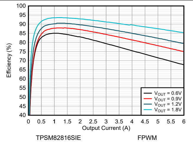
8-13. Efficiency V_{IN} = 2.7\text{ V} and T_A = 85^\circ\text{C}
