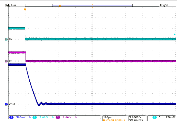
V_{OUT} = 1.8\text{ V} FPWM T_A = 25^\circ\text{C} I_{OUT} = 1\text{ A} V_{IN} = 5\text{ V} C_{SS} = 4.7\text{ nF}
