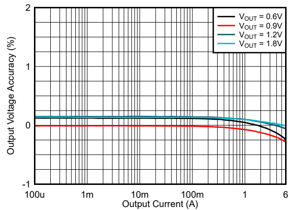
8-19. Load Regulation V IN = 2.7 V (FPWM)
