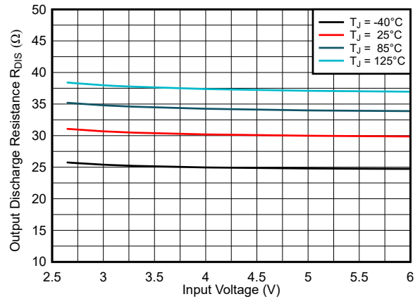
Figure 6-4. Discharge Resistance
