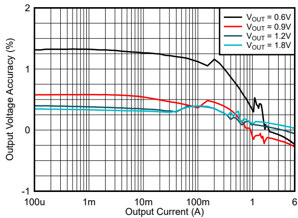
8-18. Load Regulation V IN = 2.7 V (PSM)
