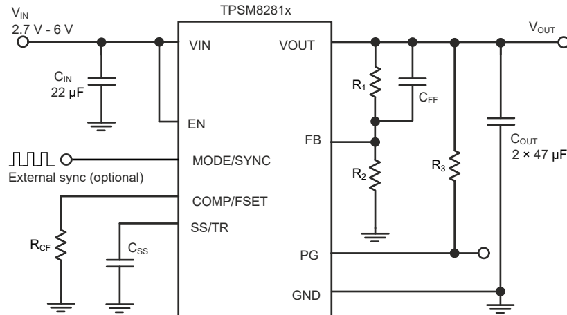
図 8-1. Typical Application Schematic
