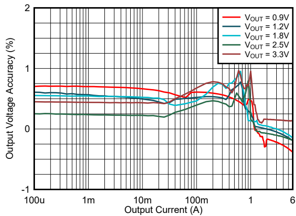
8-14. Load Regulation V IN = 5.0 V (PSM)
