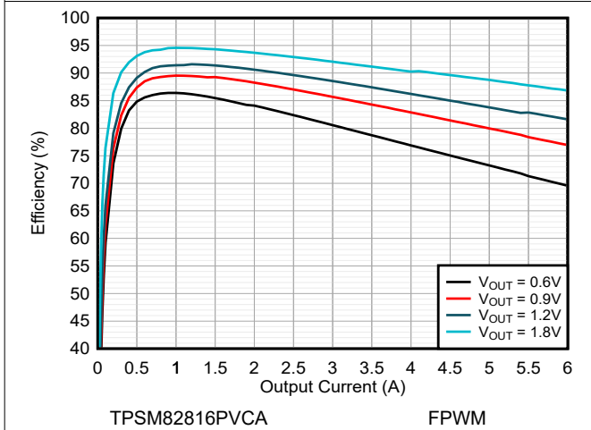
8-12. Efficiency V_{IN} = 2.7\text{ V} and T_A = 85^\circ\text{C}
