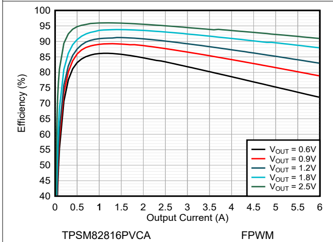
8-10. Efficiency V_{IN} = 3.3\text{ V} and T_A = 85^\circ\text{C}
