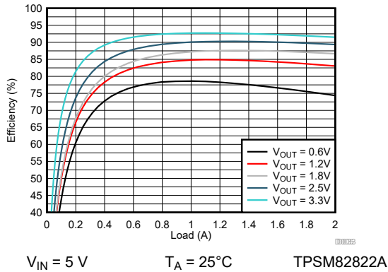
9-86. Efficiency
