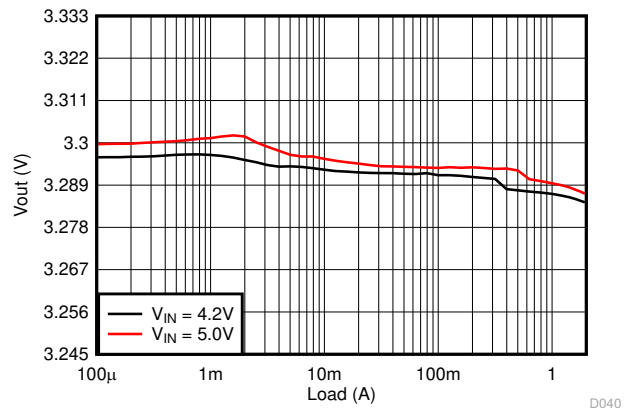
9-68. Load Regulation
