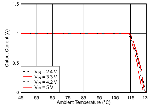
V_{OUT} = 1.2\text{ V} TPSM82821A R_{\theta JA} = 64.3^\circ\text{C/W}
