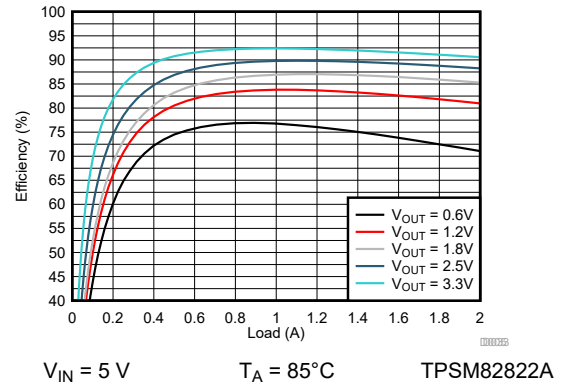
9-87. Efficiency
