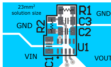
☒ 11-2. TPSM8282x/TPSM8282xA PCB Layout for the Adjustable Devices (BOM from Table 9-1 with 1 x 22-µF for C2)
