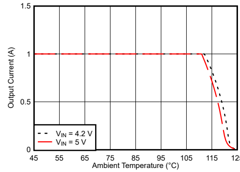
V_{OUT} = 2.5\text{ V} TPSM82821A R_{\theta JA} = 64.3^\circ\text{C/W}
