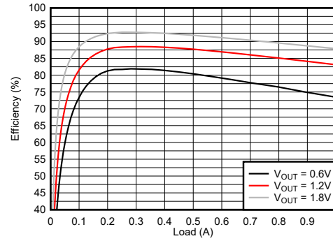
V_{IN} = 2.4\text{ V} T_A = 85^\circ\text{C} TPSM82821A
