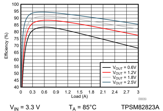
9-142. Efficiency
