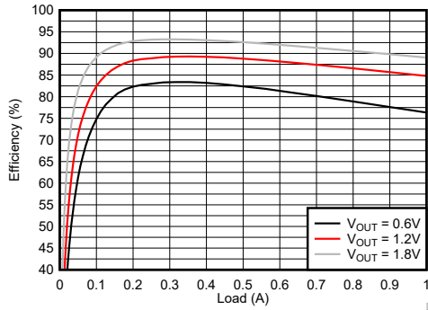
V_{IN} = 2.4\text{ V} T_A = 25^\circ\text{C} TPSM82821A
