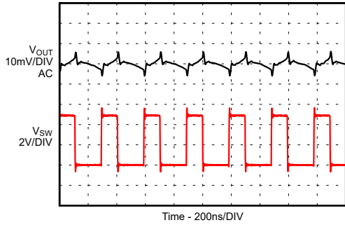
I_{OUT} = 1\text{ A} TPSM82821A
