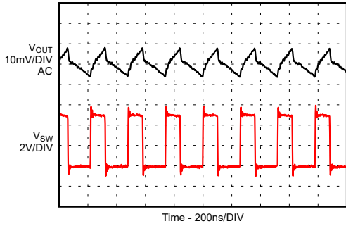
9-128. Output Ripple in PWM Mode
