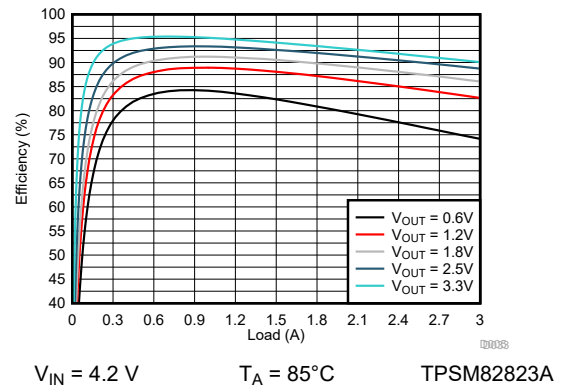
9-140. Efficiency
