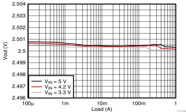
9-19. Load Regulation
