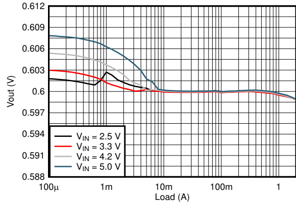
9-66. Load Regulation
