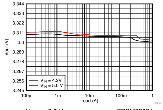
9-20. Load Regulation
