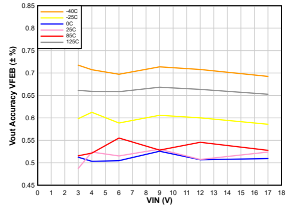
6-4. Output Voltage Accuracy – VFEB Selected
