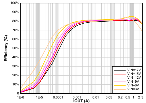
Auto PFM/PWM F_{sw} = 2.5 \text{ MHz}
