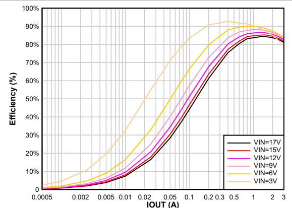
FPWM F_{sw} = 1 \text{ MHz}
