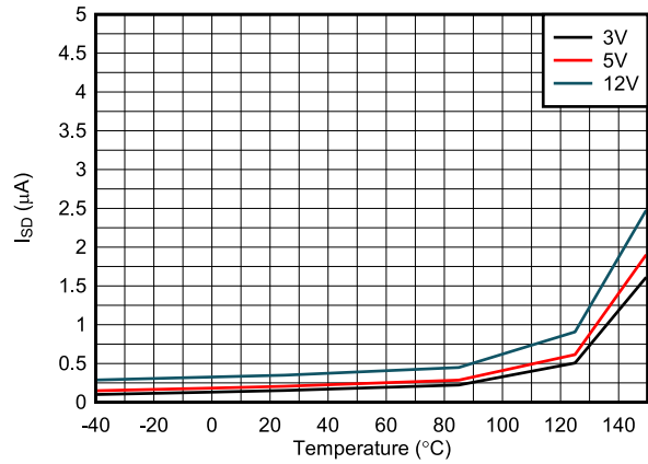
6-42. Shutdown Current vs Temperature
