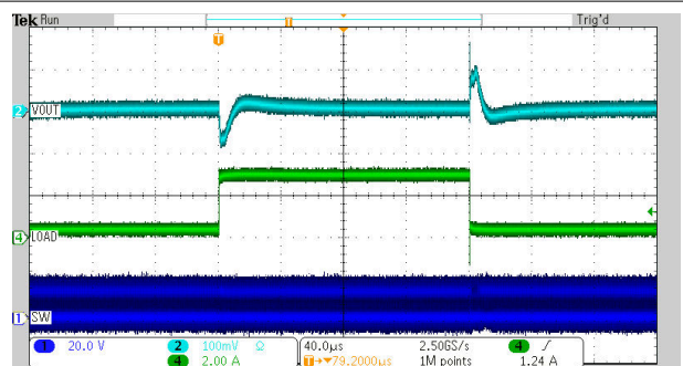
8-10. Load Transient
