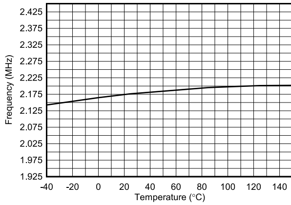
6-41. Oscillator Frequency vs Temperature
