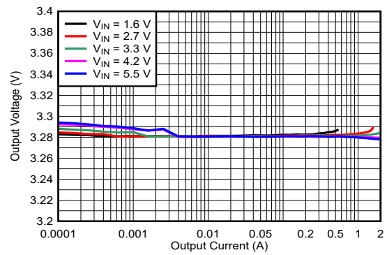
8-3. Load Regulation (FPWM)
