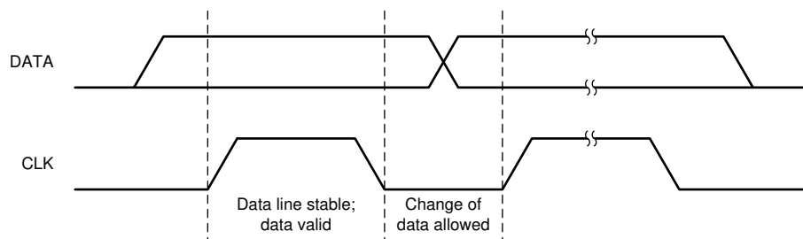
7-5. Bit Transfer on the Serial Interface
