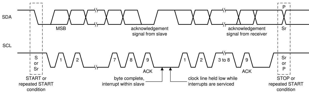
Figure 7-7. Bus Protocol
