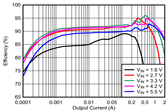
8-2. Efficiency vs Output Current (FPWM)
