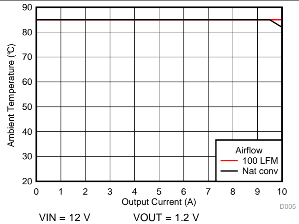
⊗ 6. Safe Operating Area
