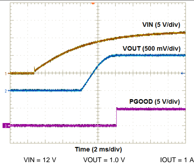
⊗ 7. VIN Start-up Waveforms
