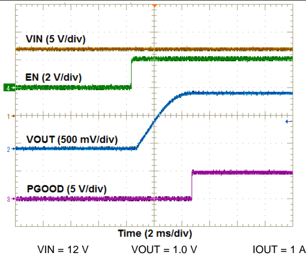
⊗ 9. EN Start-up Waveforms
