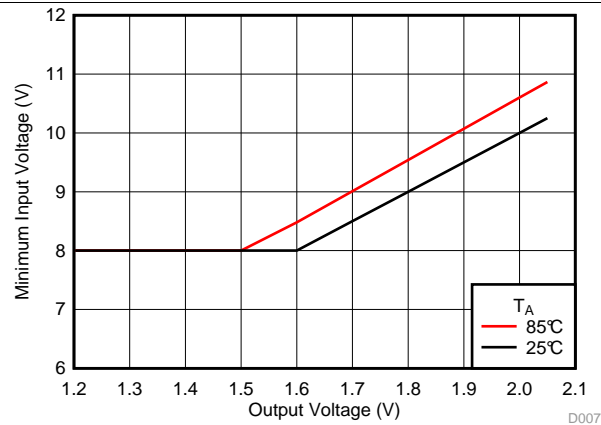
11. Minimum Input Voltage
