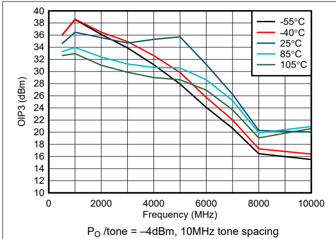
5-7. OIP3 Across Temperature
