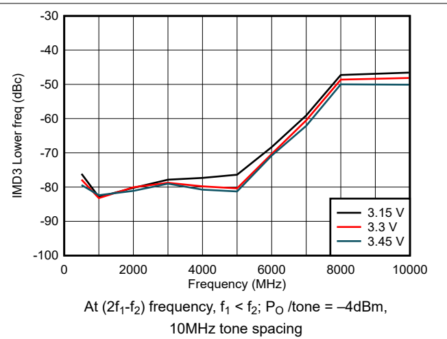
5-10. IMD3 Lower Across V_{DD}
