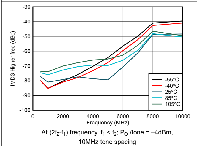
5-11. IMD3 Higher Across Temperature
