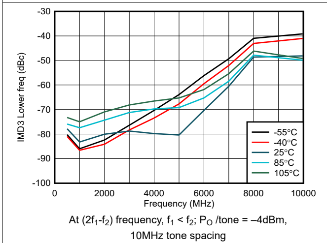
5-9. IMD3 Lower Across Temperature
