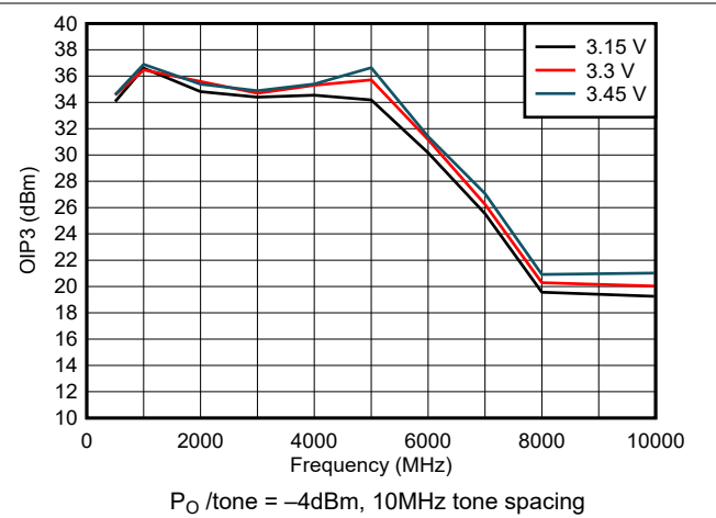
5-8. OIP3 Across V_{DD}
