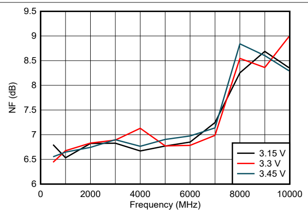
图 5-30. NF Across V_{DD}
