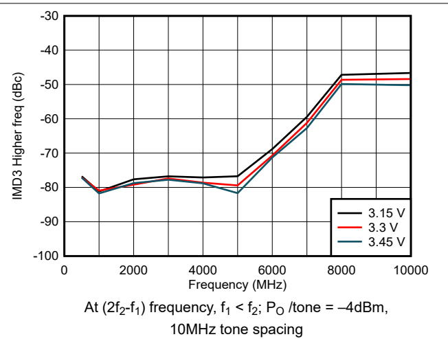
5-12. IMD3 Higher Across V_{DD}
