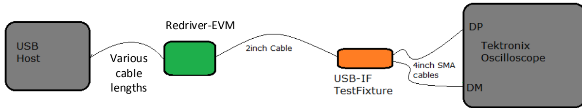
図 8-2. Near End Eye Measurement Set-Up With Pre-Channel Cable
