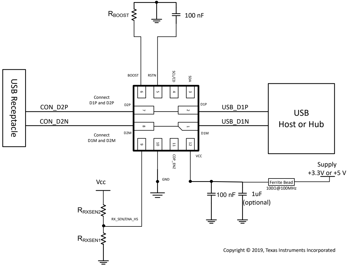
8-1. TUSB216 Reference Schematic (Design Example with CDP disabled), CDP_ENZ Can Be Left Floating but an Option for a Decoupling Capacitor of 0.1 \mu F is Recommended So the Design is Compatible with Older Devices: TUSB211, TUSB212, TUSB214
