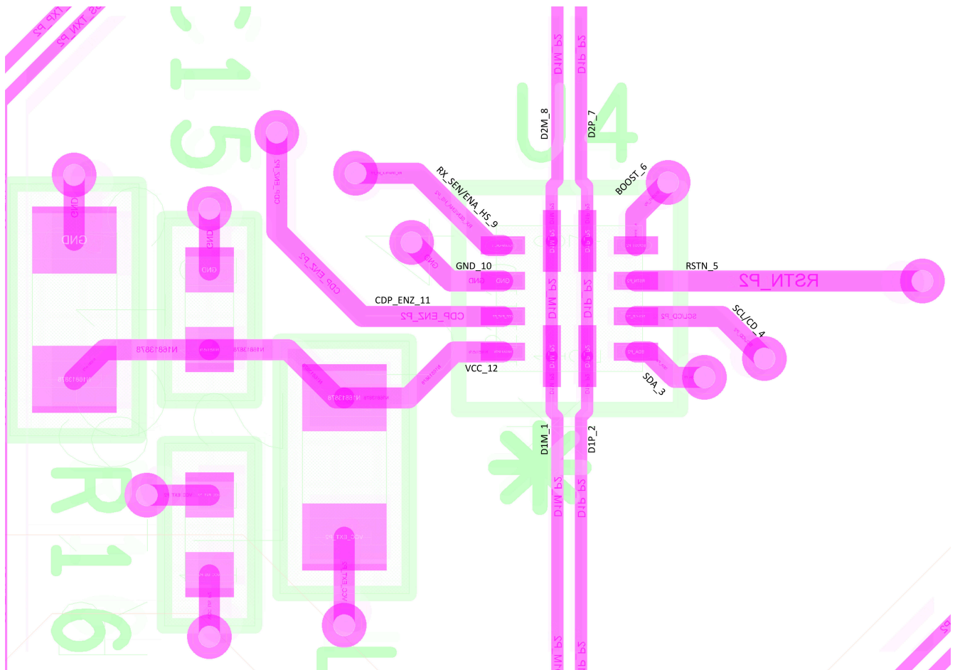
☒ 8-22. Layout Example
