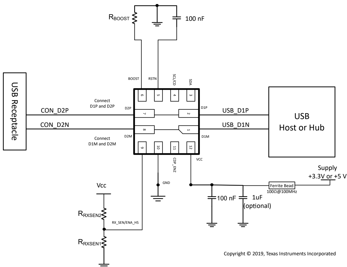
図 8-1. TUSB216 Reference Schematic (Design Example with CDP disabled), CDP_ENZ Can Be Left Floating but an Option for a Decoupling Capacitor of 0.1 \mu F is Recommended So the Design is Compatible with Older Devices: TUSB211, TUSB212, TUSB214
