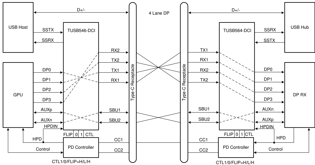
8-9. Four Lane DP – With Flip (CTL1 = H, CTL0 = L, FLIP = H)
