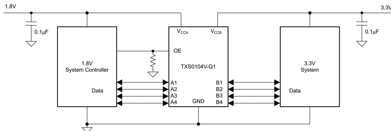
図 8-1. Application Schematic
