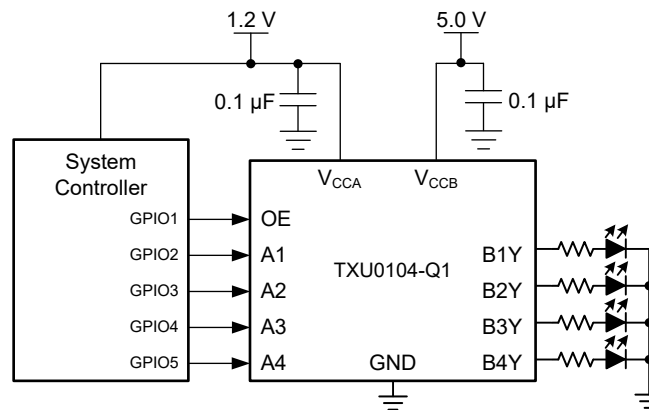
図 10-1. TXU0104-Q1 LED Driver Application
