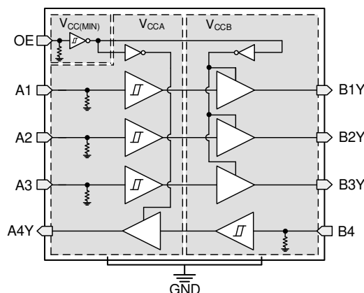
FIG 5-2. TXU0304-Q1 Functional Block Diagram
