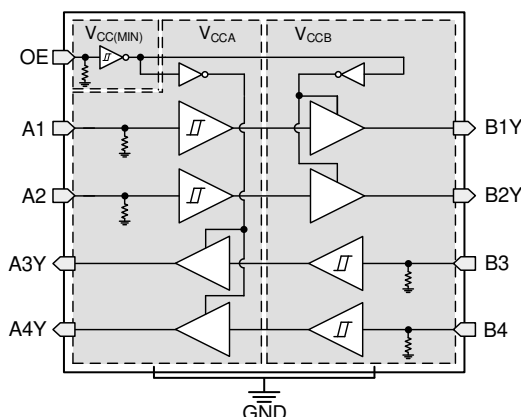
FIG 5-1. TXU0204-Q1 Functional Block Diagram
