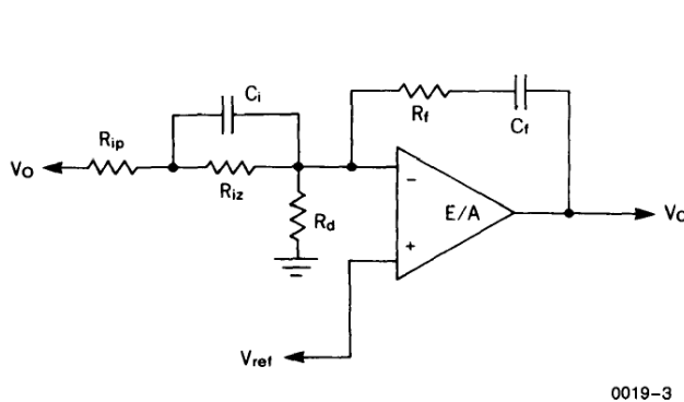
A. Direct duty cycle control
