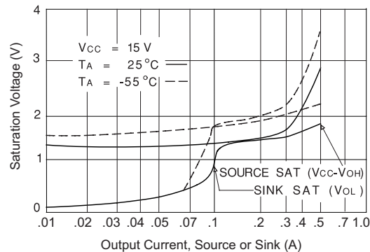
Figure 1. Output Saturation Characteristics
