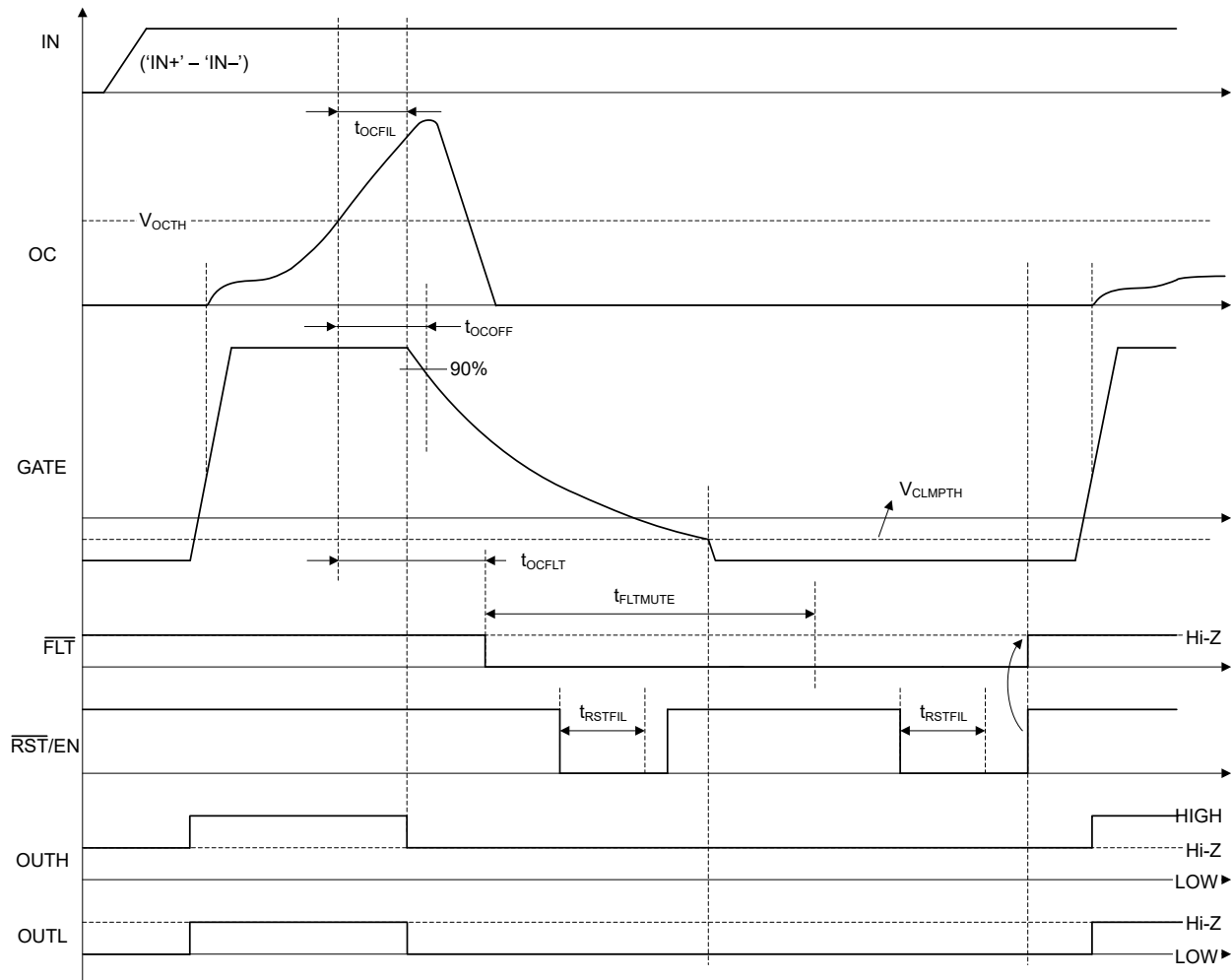
7-10. OC Protection with Soft Turn-OFF
