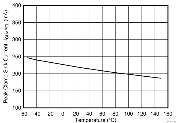
图 6-22. I_{CLMPEL} Miller Clamp Sink Current vs Temperature
