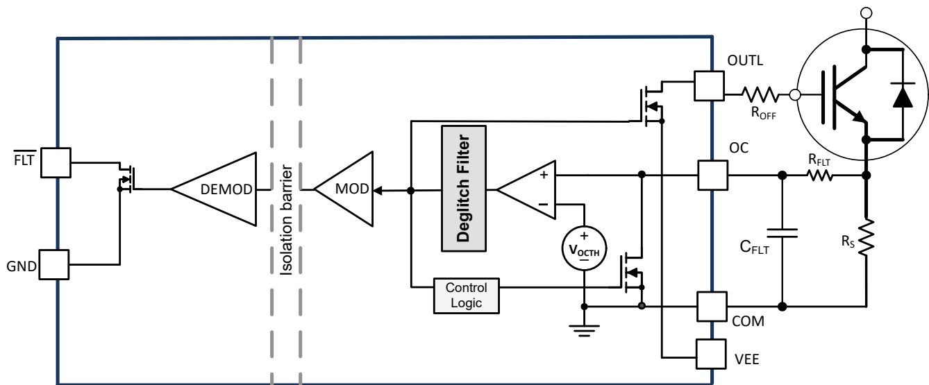
図 8-5. Overcurrent and Short Circuit Protection
