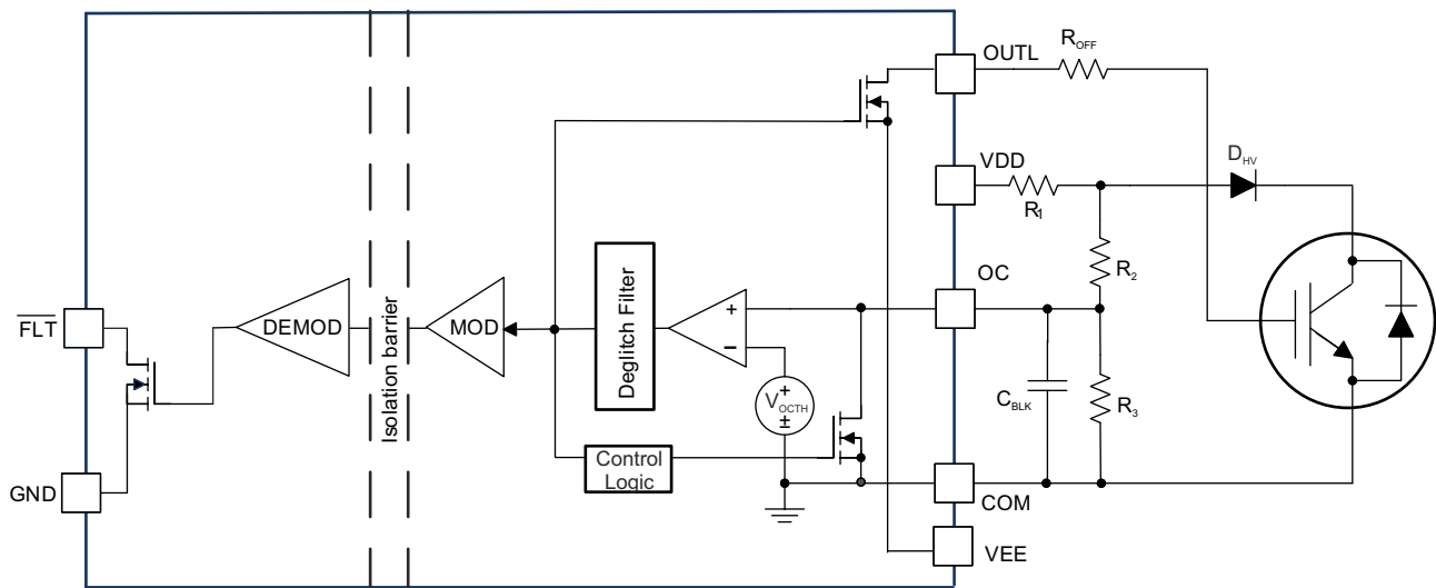
図 9-9. Overcurrent and Short Circuit Protection Based on Desaturation Circuit
