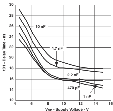
図 6-2. Delay Time ( t_{D1} ) vs Supply Voltage
