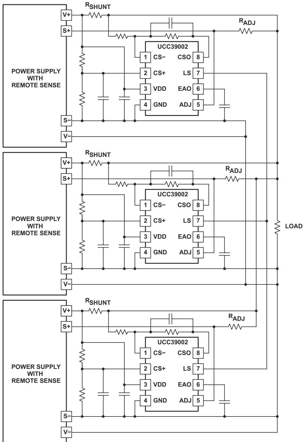
7-3. Three-Module Sharing Example with High-Side Current-Sensing, System V_{OUT} < 13.5V
