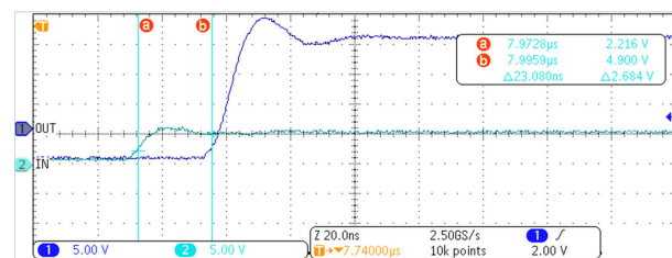
図 7-3. UCC57102Z Rising (Turn-On) Propagation Delay
