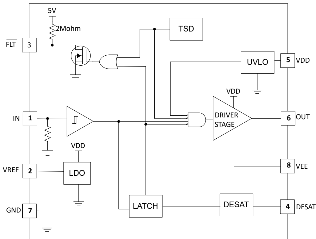
図 6-1. UCC57102Z Simplified Functional Block Diagram
