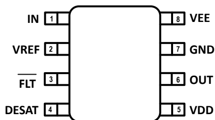
図 4-1. UCC57102Z D Package SOIC-8 Top View
