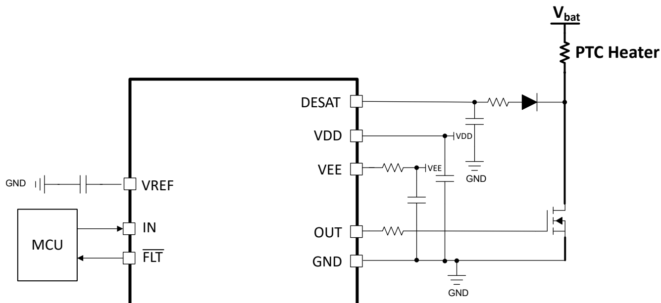
図 7-1. UCC57102Z Used in a PTC Heater Application
