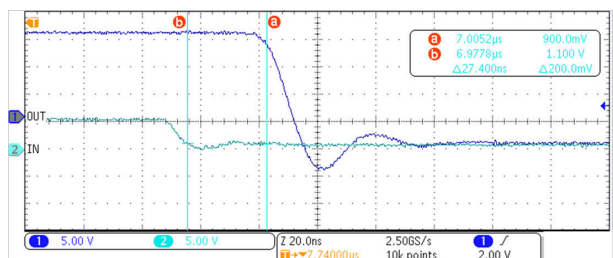
図 7-4. UCC57102Z Falling (Turn-Off) Propagation Delay
