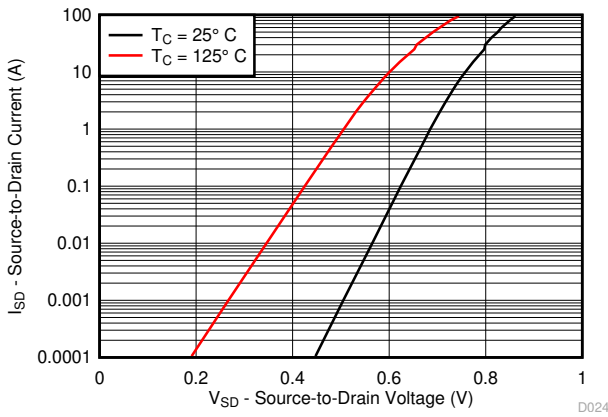
4-15. MOSFET Body Diode Forward Voltage
