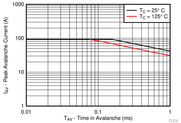
4-16. MOSFET Single Pulse Unclamped Inductive Switching
