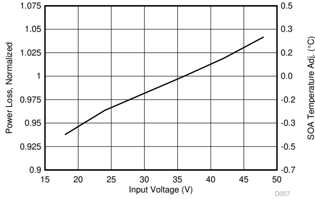
4-5. Normalized Power Loss vs Input Voltage
