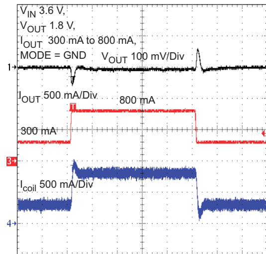
Figure 16. PWM Load Transient
