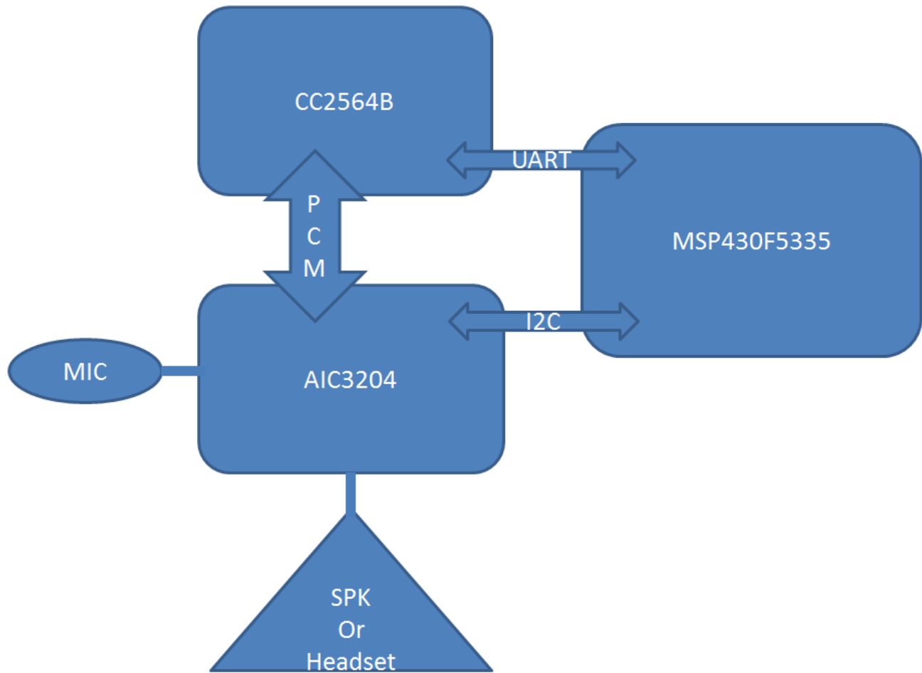
Figure 2. System Architecture
