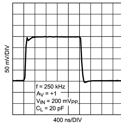
FIGURE 2. Small Signal Step Response with Gain = 1
