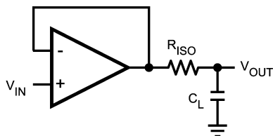
FIGURE 1. Isolating Capacitive Load
