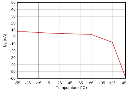
5-50. TPS73601 I_{FB} vs Temperature
