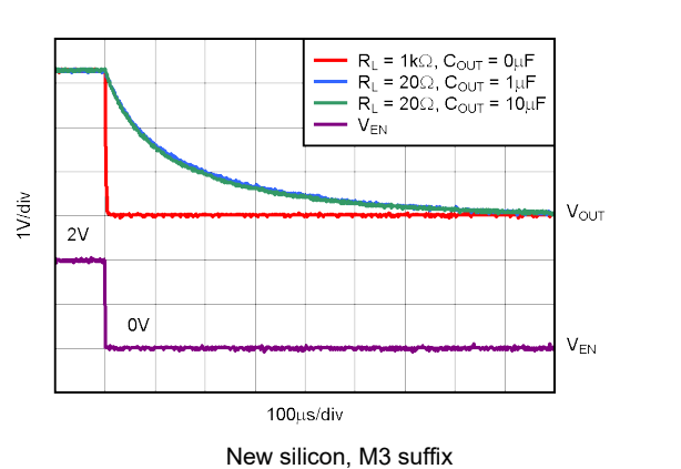
5-42. TPS73633 Turn-Off Response
