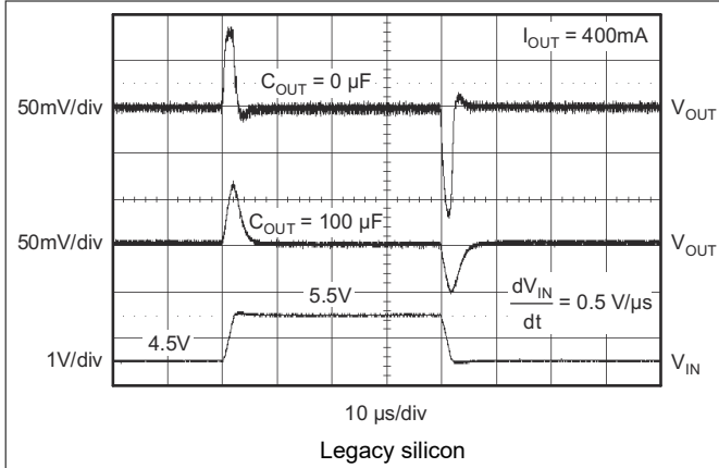
5-37. TPS73633 Line Transient Response
