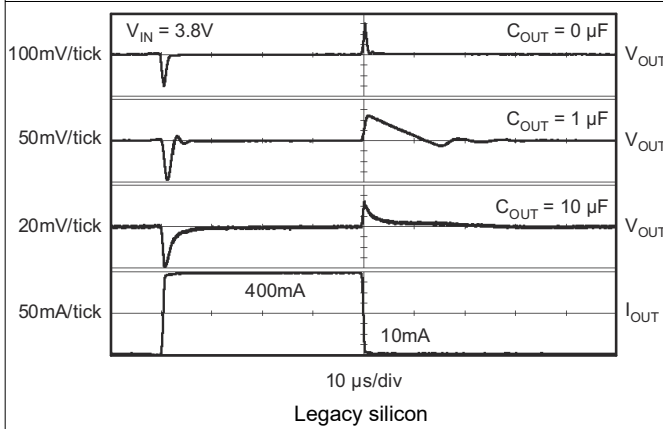
7-5. TPS73633 Load Transient Response
