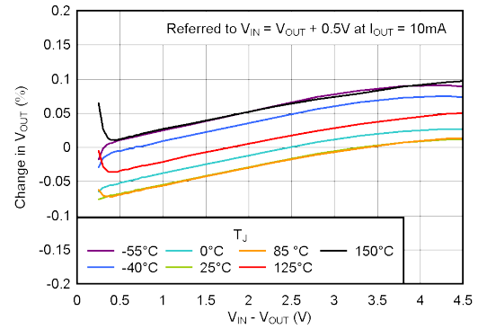
New silicon, M3 suffix 图 5-4. Line Regulation
