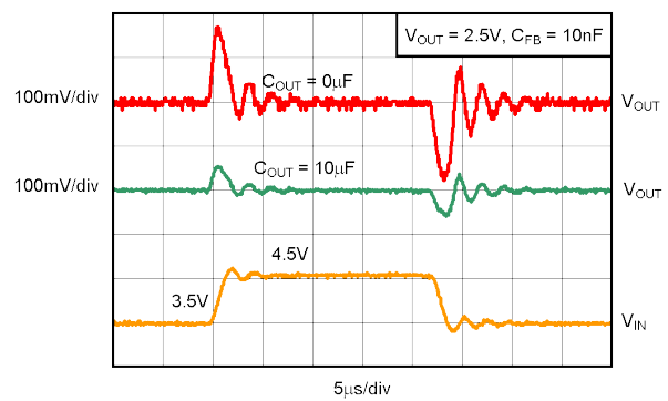
5-54. TPS73601 Line Transient, Adjustable Version
