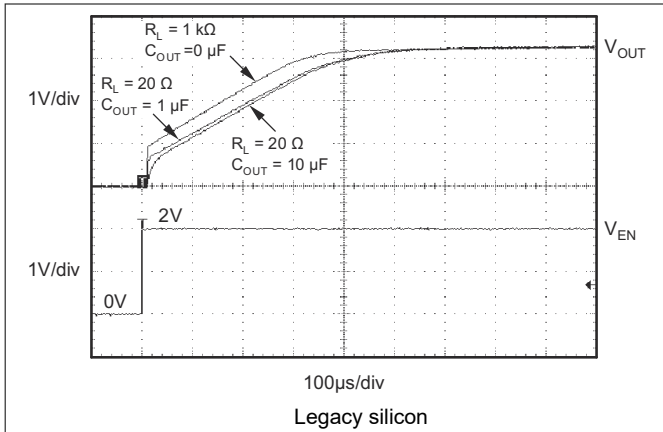
7-3. TPS73633 Turn-On Response
