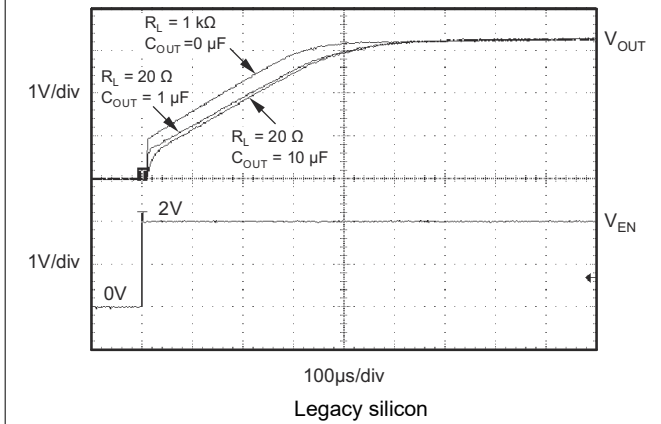
5-39. TPS73633 Turn-On Response
