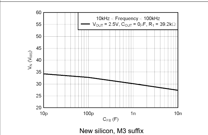
7-8. TPS73601 RMS Noise Voltage vs C FB
