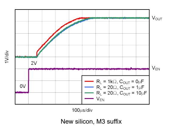
5-40. TPS73633 Turn-On Response
