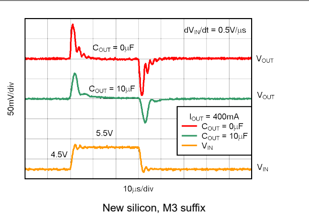
5-38. TPS73633 Line Transient Response
