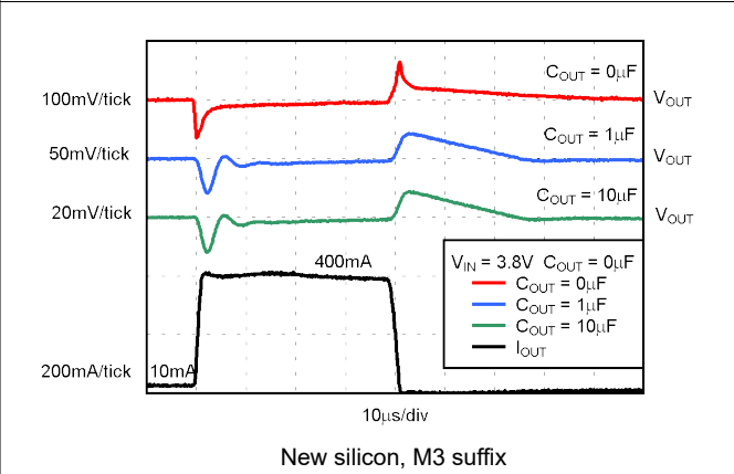
7-6. TPS73633 Load Transient Response
