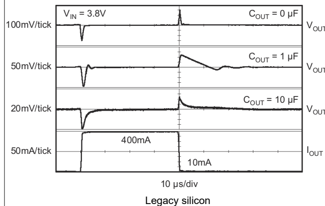
5-35. TPS73633 Load Transient Response
