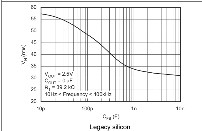
7-7. TPS73601 RMS Noise Voltage vs C FB
