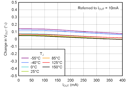
New silicon, M3 suffix 图 5-2. Load Regulation
