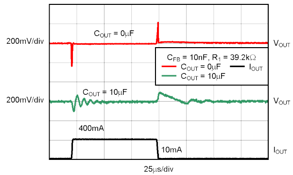
5-52. TPS73601 Load Transient, Adjustable Version
