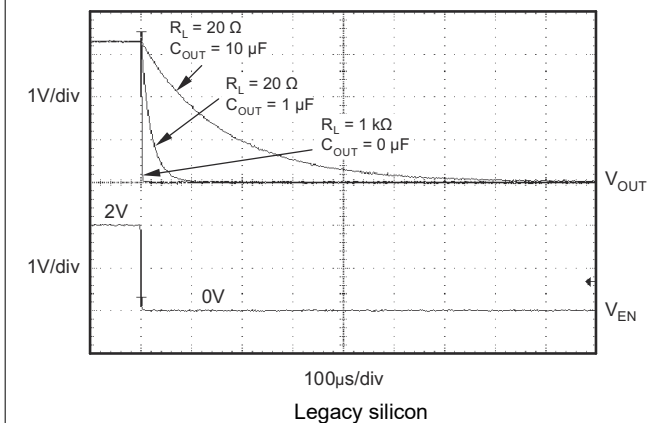
5-41. TPS73633 Turn-Off Response
