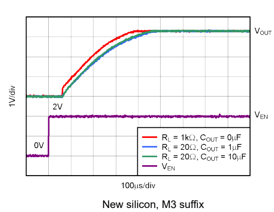
Figure 5-40. TPS73233 Turn-On Response
