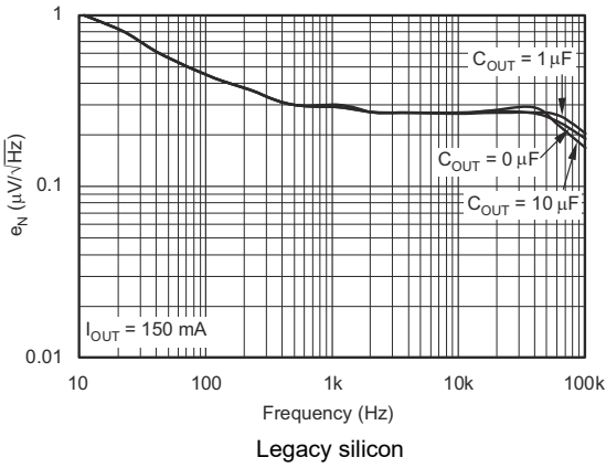
5-27. Noise Spectral Density C_{NR} = 0\mu\text{F}
