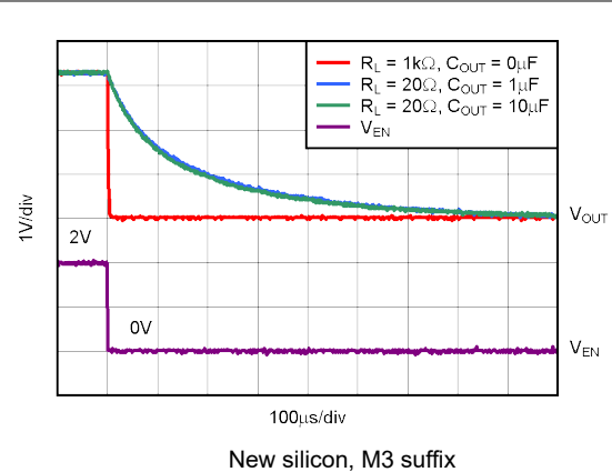
Figure 5-42. TPS73233 Turn-Off Response
