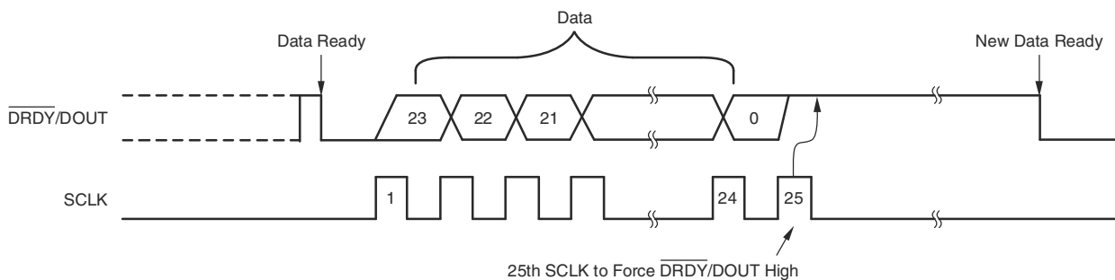
Figure 8-10. Data Retrieval With \overline{\text{DRDY}}/\text{DOUT} Forced High Afterwards
