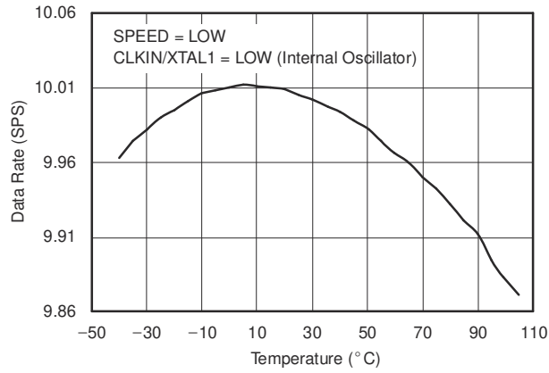
6-25. Data Rate vs Temperature
