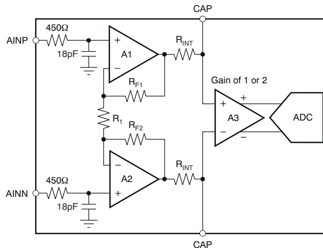
Figure 8-2. Simplified Diagram of the PGA
