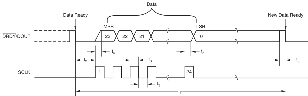
Figure 8-9. Data Retrieval Timing
