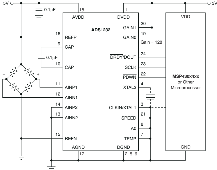
図 9-1. Weigh-Scale Application
