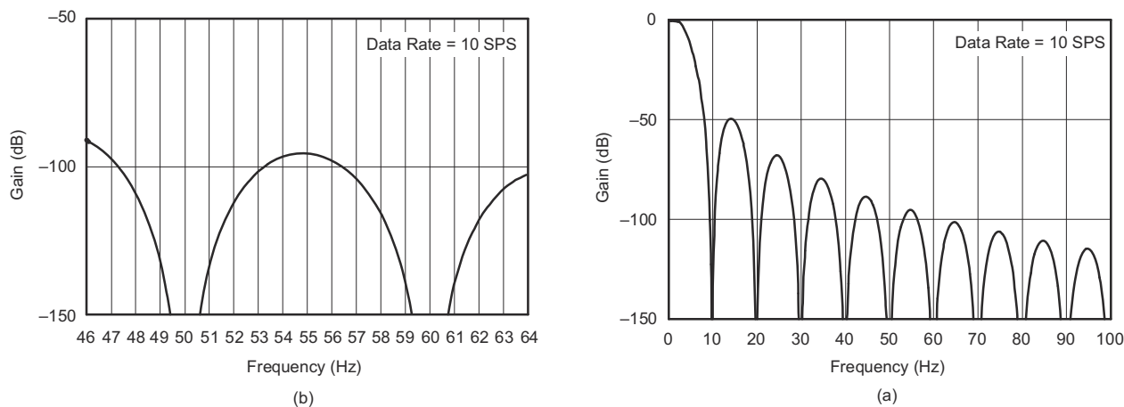
Figure 8-6. Digital Filter Frequency Response to 100 Hz
