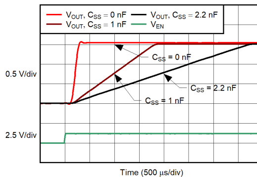
Figure 7-6. Turn-On Response
