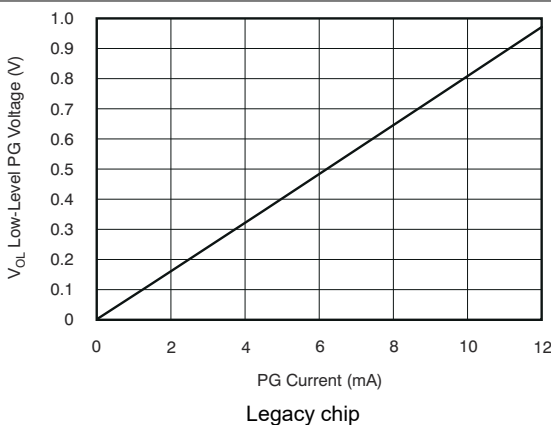
Figure 5-29. Low-Level PG Voltage vs Current
