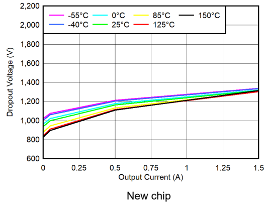
5-14. V BIAS Dropout Voltage vs I OUT and Temperature (T J )
