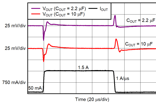
Figure 7-5. Output Load Transient Response
