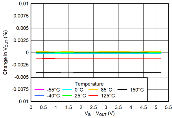
6-22. V IN Line Regulation
