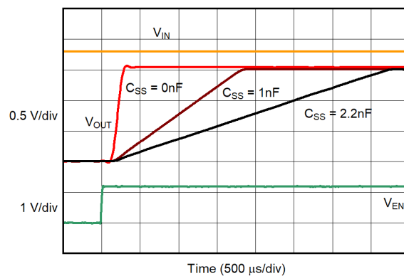
6-44. Turn-On Response
