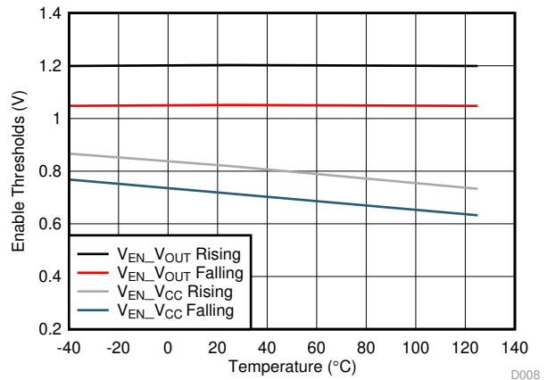
Figure 8. Enable Threshold
