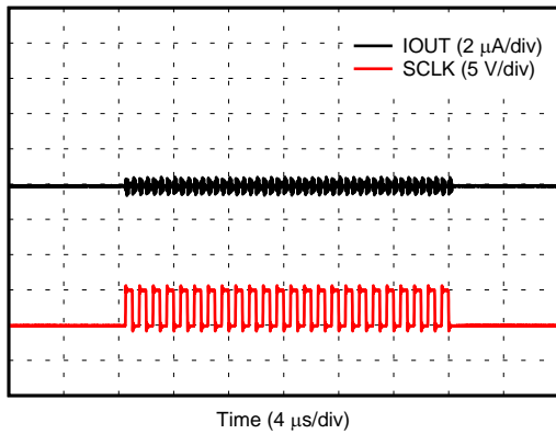
70. IOUT Digital Feed-Through
