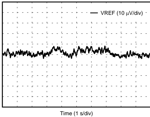
76. Internal Reference Voltage Noise (DC/DC Disabled)
