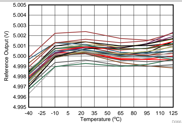
71. Internal Reference Voltage vs Temperature
