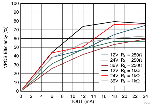
79. IOOUT VPOS Efficiency
