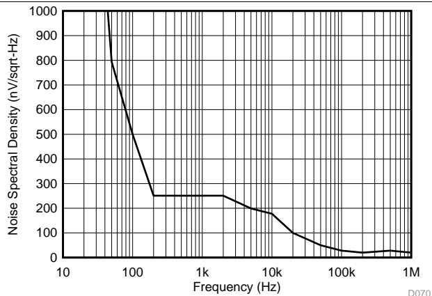
74. Internal Reference Voltage Noise Spectral Density (DC/DC Disabled)
