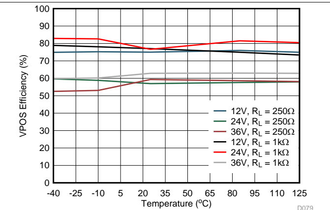
FIG 81. VPOS Efficiency vs Temperature
