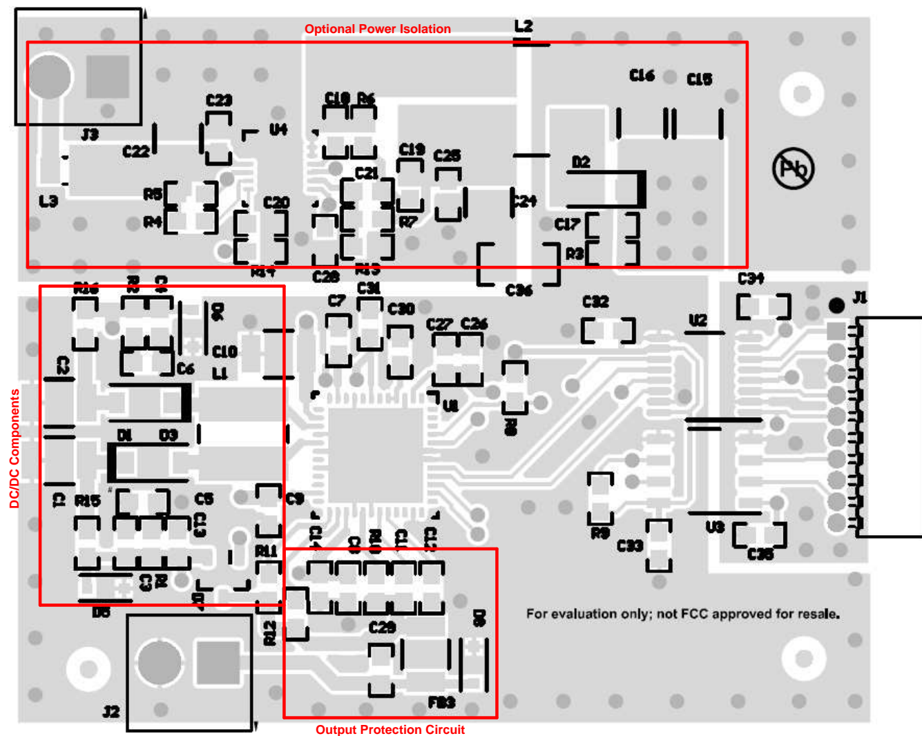
☒ 132. Application Example Layout
