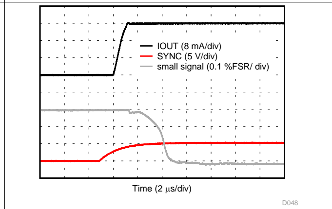
图 55. IOUT Settling Time, Rising Signal
