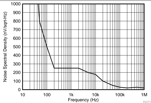
75. Internal Reference Voltage Noise Spectral Density (DC/DC Enabled)
