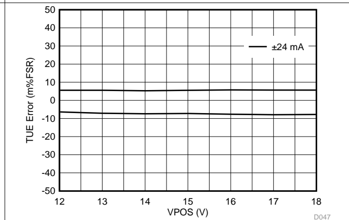
图 53. IOUT Bipolar Range TUE vs VPOS
