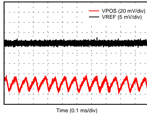
77. Internal Reference Voltage DC/DC Ripple
