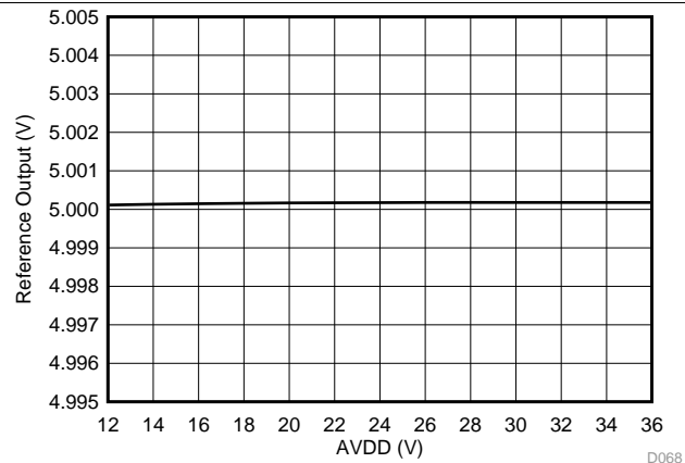
73. Internal Reference Voltage vs AVDD
