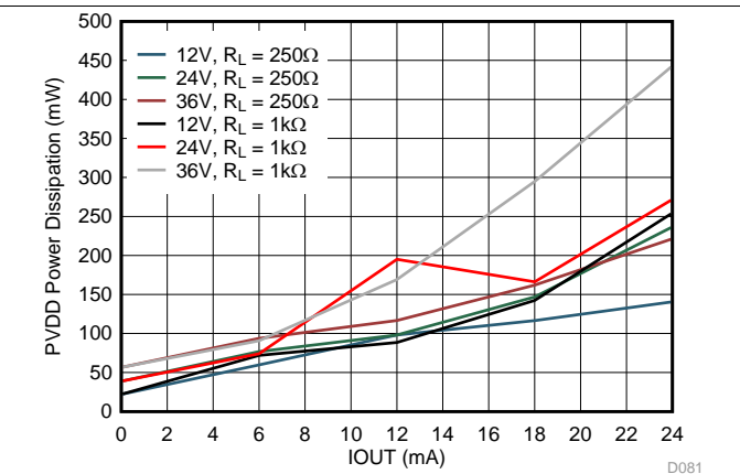
FIG 83. IOUT Power Dissipation vs Load
