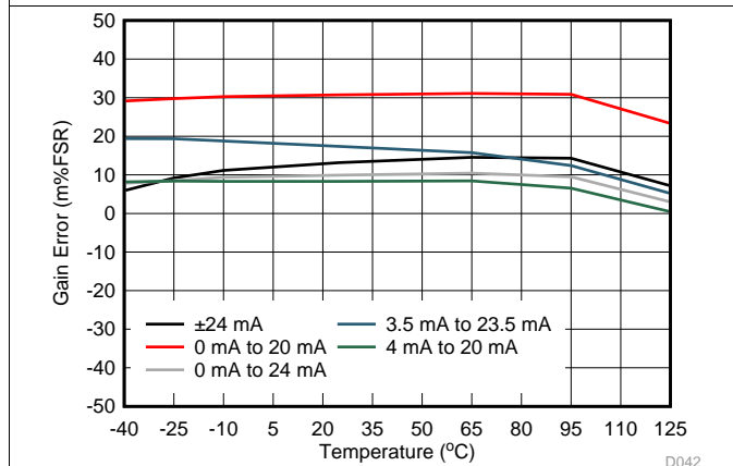
图 46. IOUT Gain Error vs Temperature
