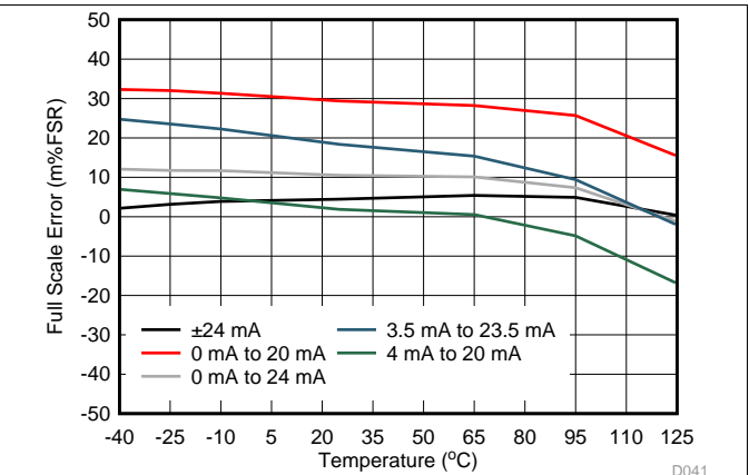
图 45. IOUT Full-Scale Error vs Temperature
