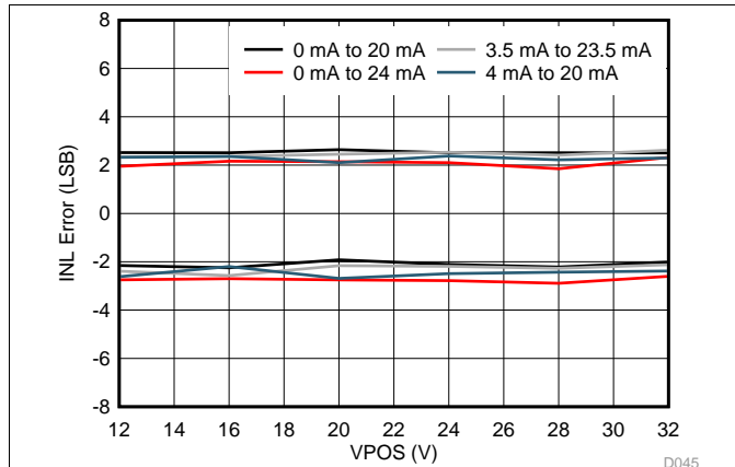
图 50. IOUT Unipolar Ranges INL vs VPOS
