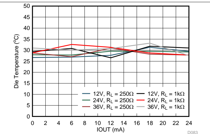
FIG 85. IOUT Die Temperature vs Load
