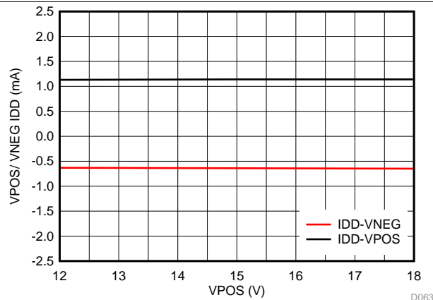
69. IOUT Quiescent Current vs VPOS
