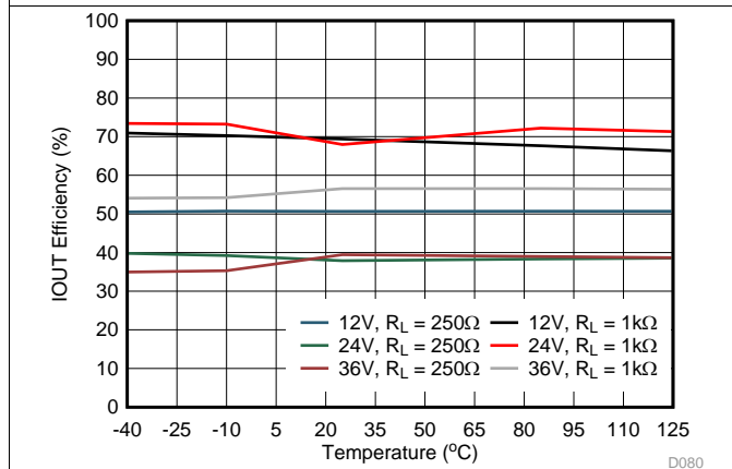
FIG 82. IOUT DC/DC Efficiency vs Temperature
