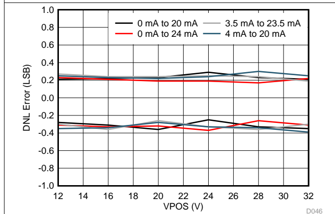
图 52. IOUT Unipolar Ranges DNL vs VPOS
