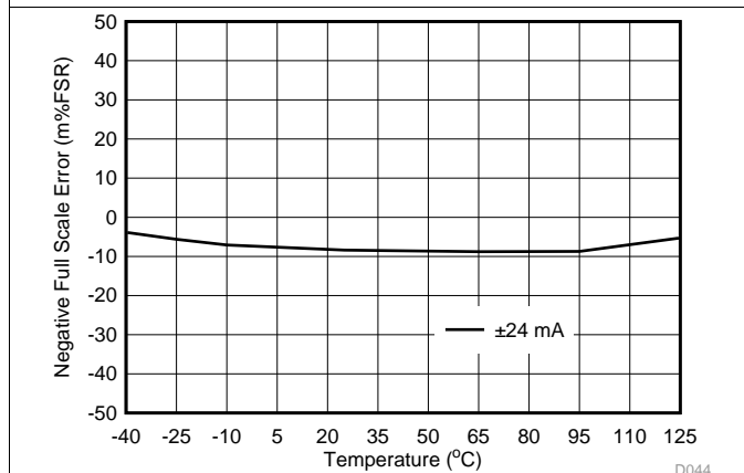
图 48. IOUT Negative Full-Scale Error vs Temperature
