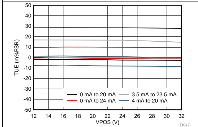
图 54. IOUT Unipolar Ranges TUE vs VPOS
