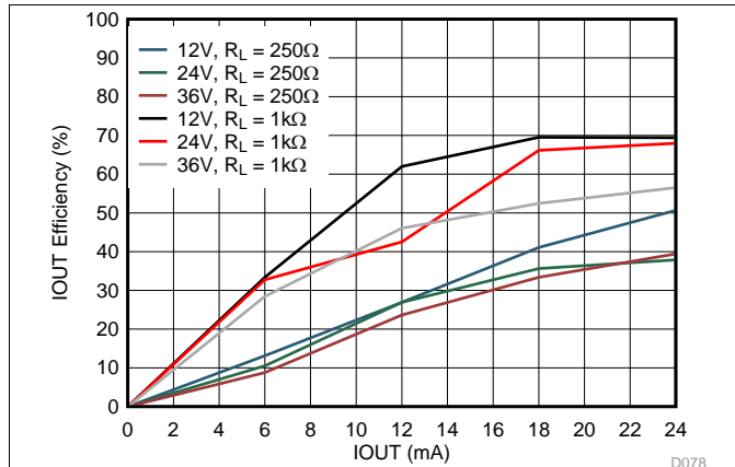
FIG 80. IOUT DC/DC Efficiency
