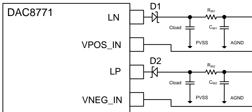
Figure 100. Buck-Boost Converter Positive and Negative Outputs
